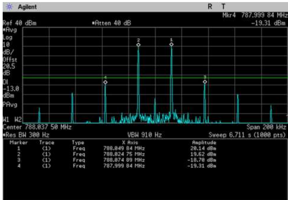
Intermodulation _UL_788-798-LC-AGC_ 788.0375MHz_25kHz
