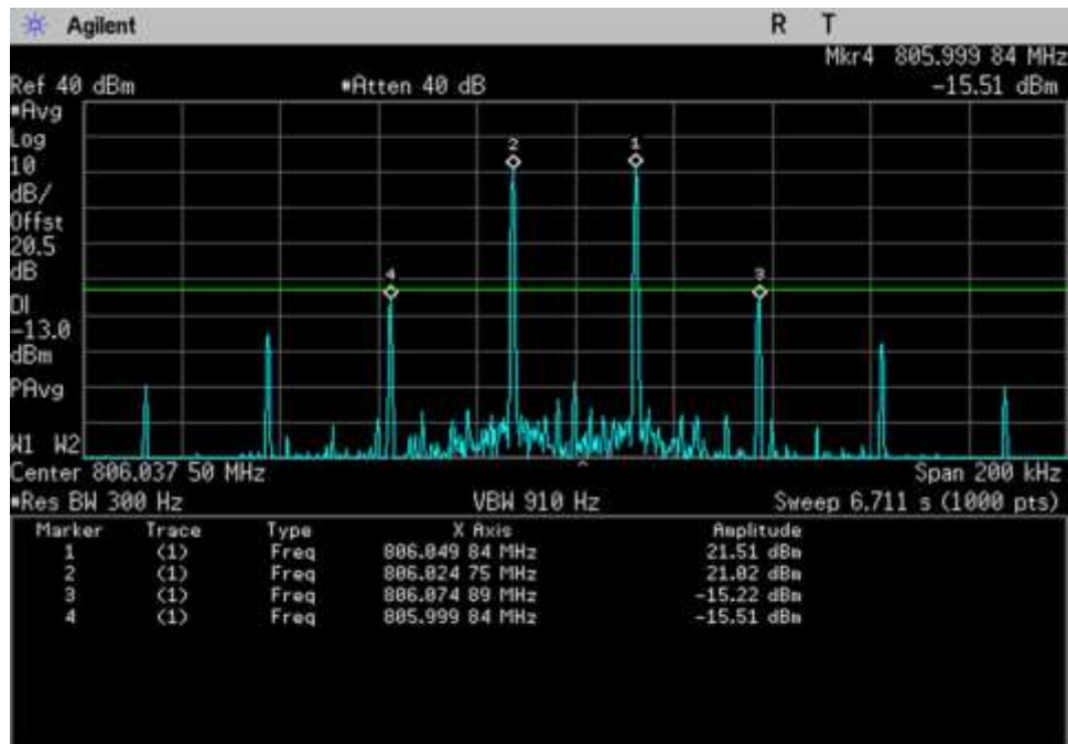
Intermodulation _UL_806-816-LC-AGC_ 806.0375MHz_25kHz
