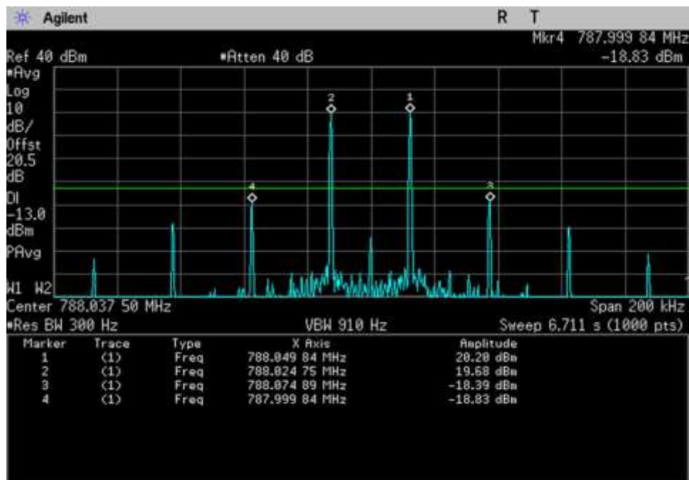
Intermodulation _UL_788-798-LC-AGC+3_ 788.0375MHz_25kHz
