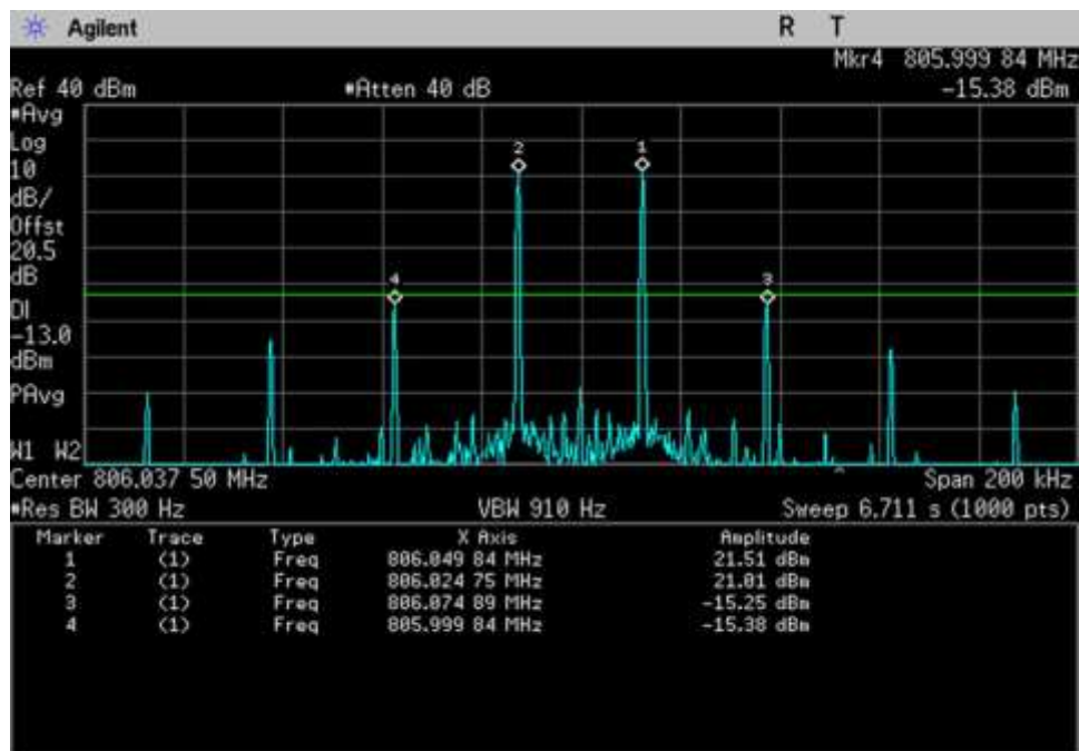
Intermodulation _UL_806-816-LC-AGC+3_ 806.0375MHz_25kHz
