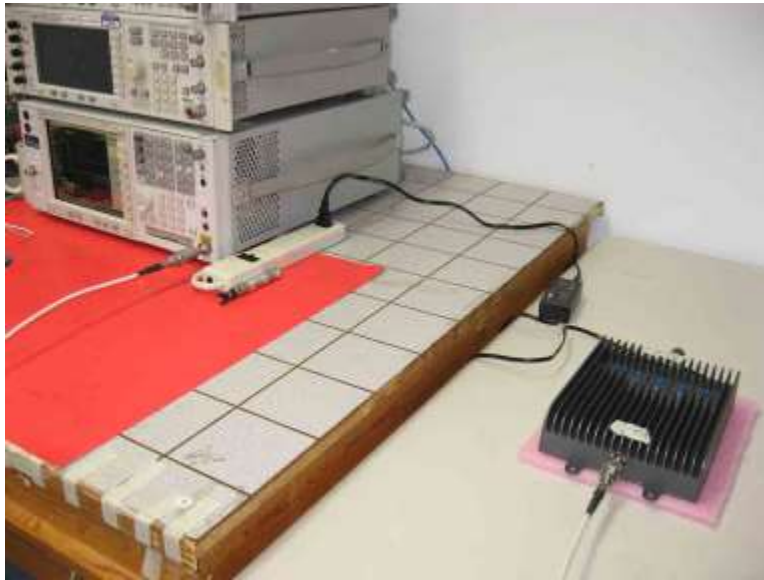
7.8 Test Setup
