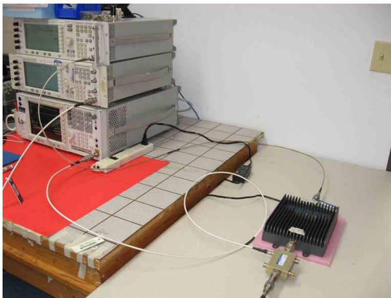
7.9 Test Setup
