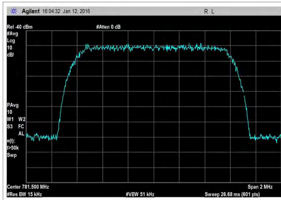
7.10_OBW_UL_776-787MHz_CDMA
