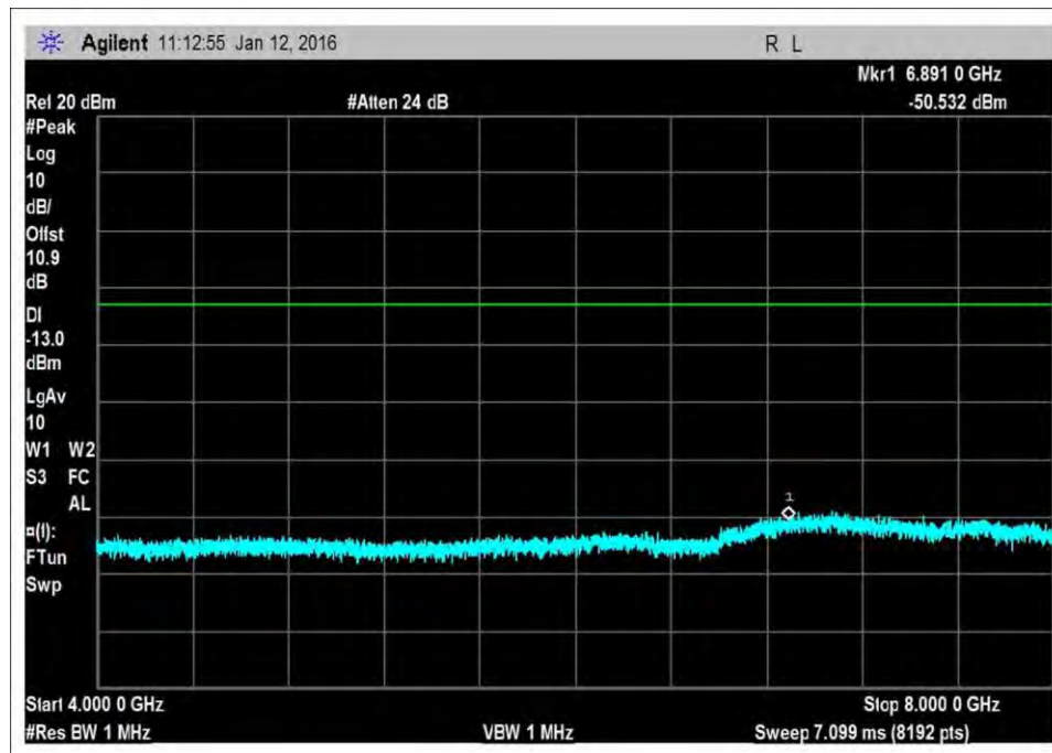
DL_2110-2155R2
