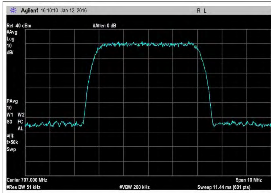
7.10_OBW_UL_698-716MHz_WCDMA
