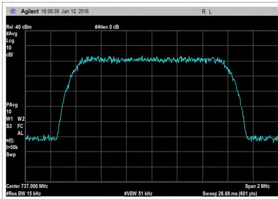
7.10_OBW_DL_728-746MHz_CDMA
