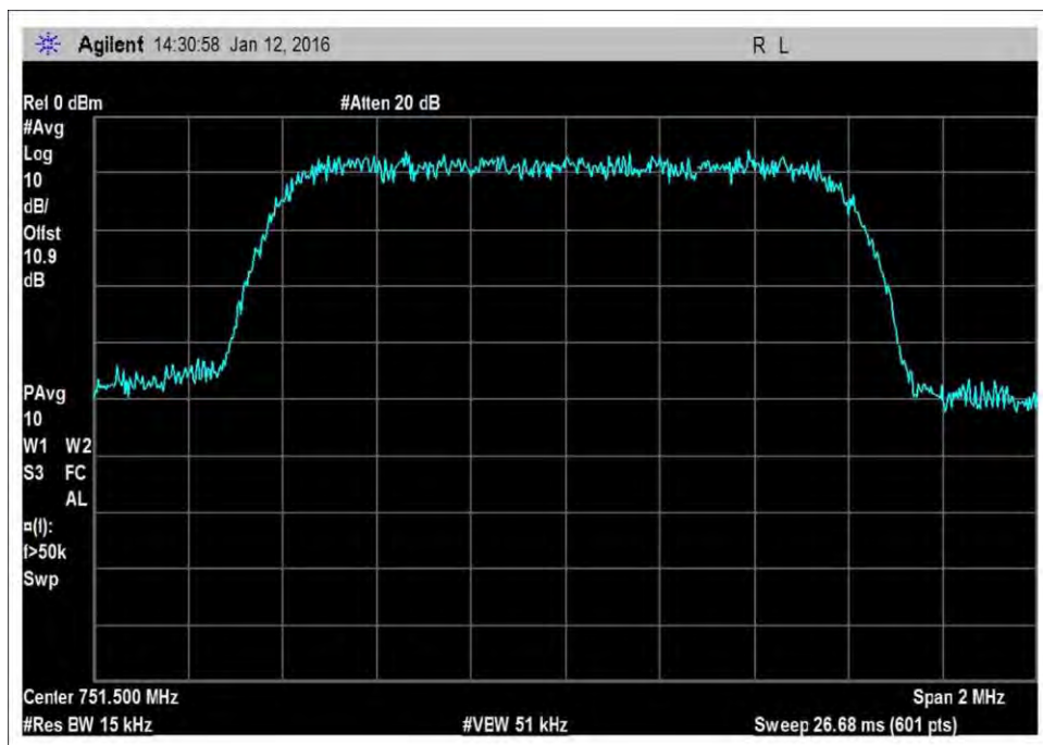
7.10_OBW_DL_746-757MHz_CDMA
