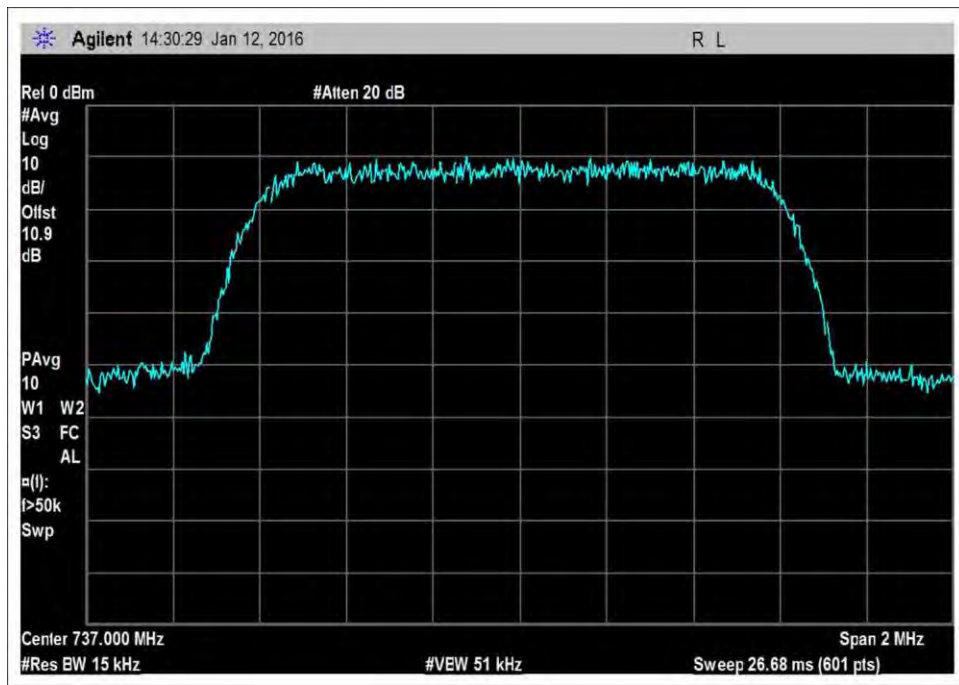
7.10_OBW_DL_728-746MHz_CDMA
