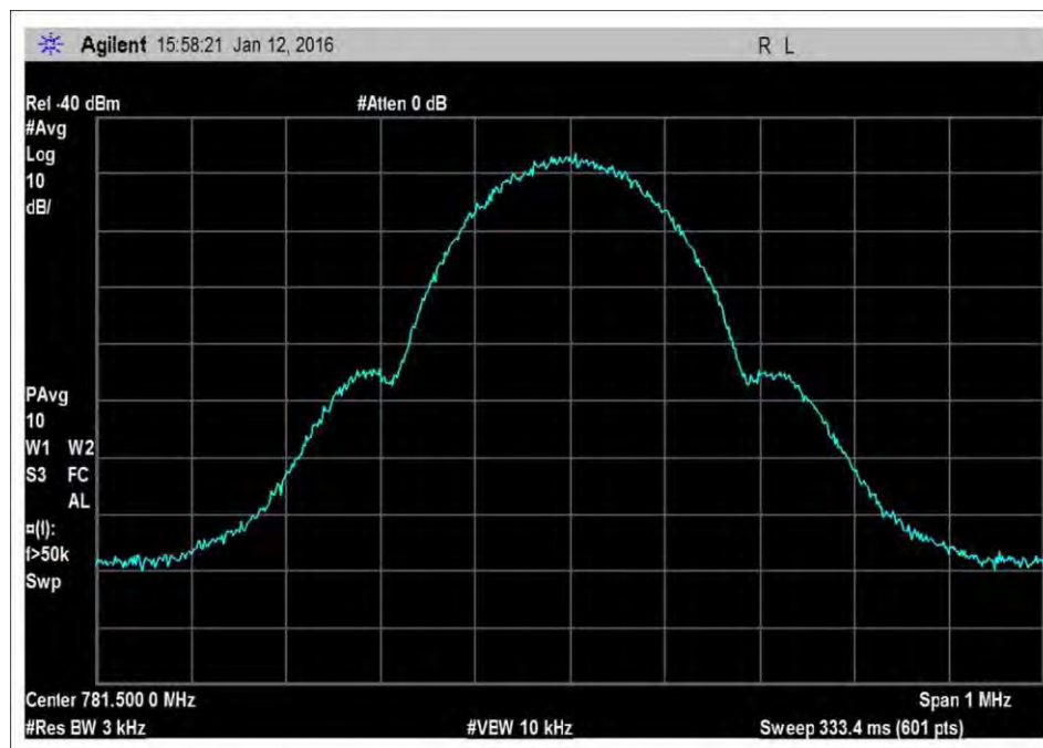
7.10_OBW_UL_776-787MHz_GSM
