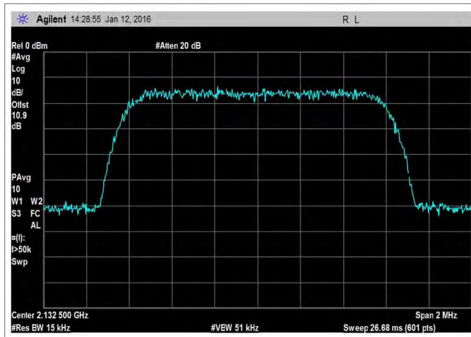
7.10_OBW_DL_2110-2155MHz_CDMA
