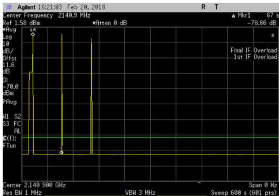
DL_2110-2155_600sec_ 2140.9MHz
