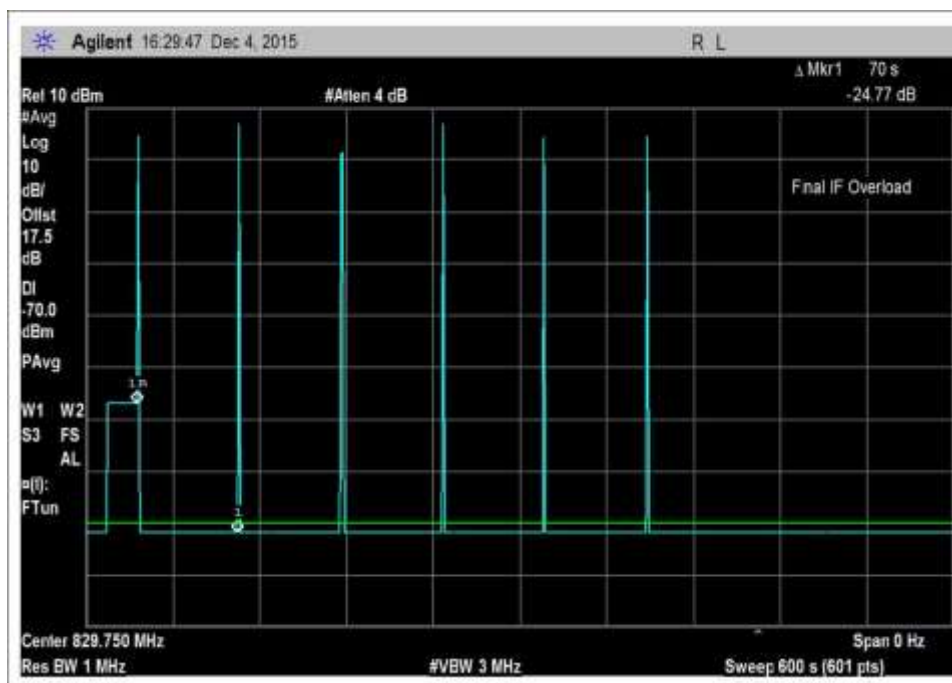
7.11_osc_UL-824-849MHz-600sec
