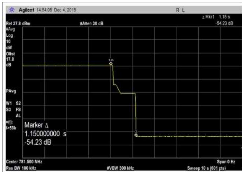
7.9.2_VarULGainTiming_UL_776-787MHz
