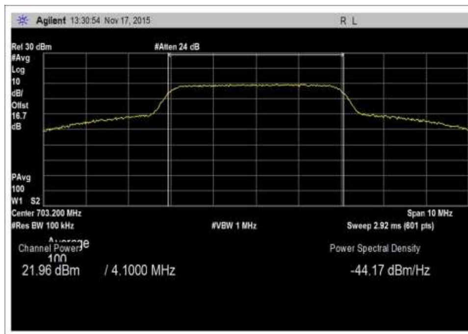
7.2_Power_UL_698-716_AWGN-Max
