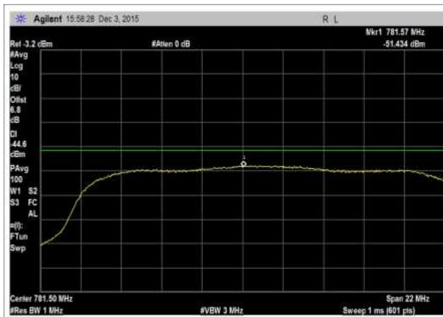
7.7_Noise_UL_776-787MHz
