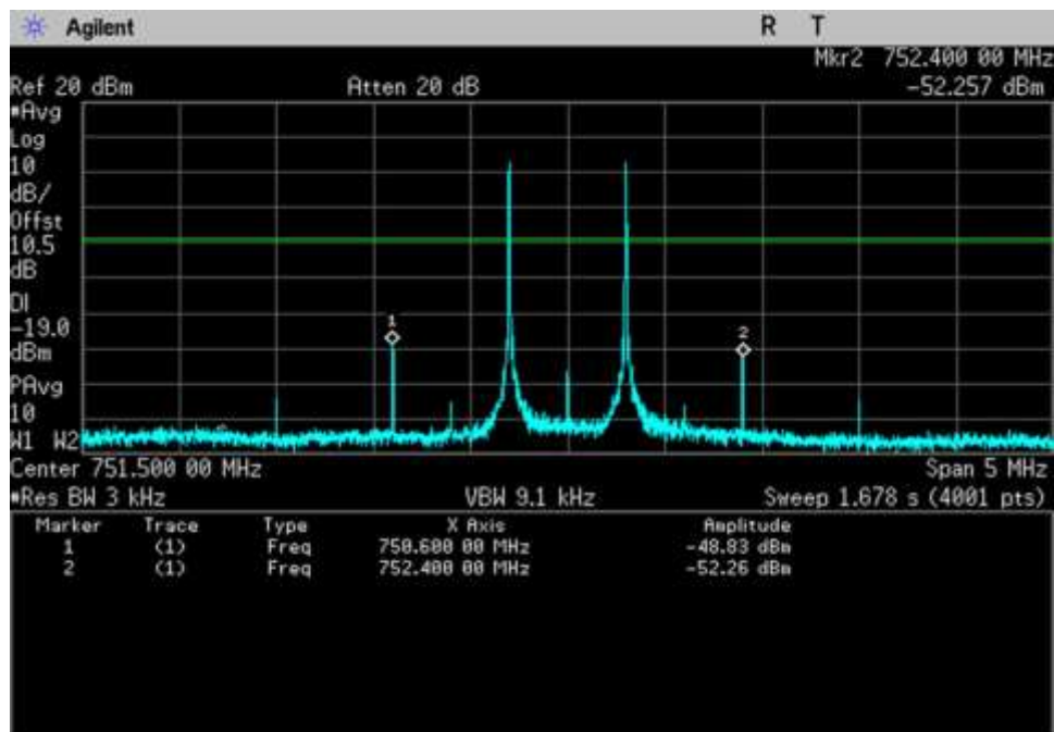
7.4_Intermod_DL_746-757MHz
