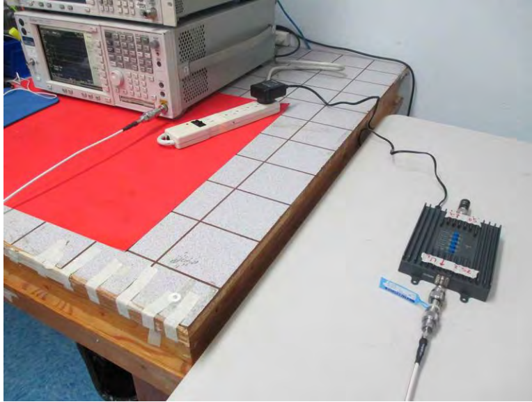
7.8 Test Setup
