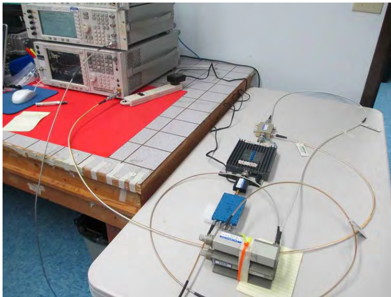
7.11.3 Test Setup
