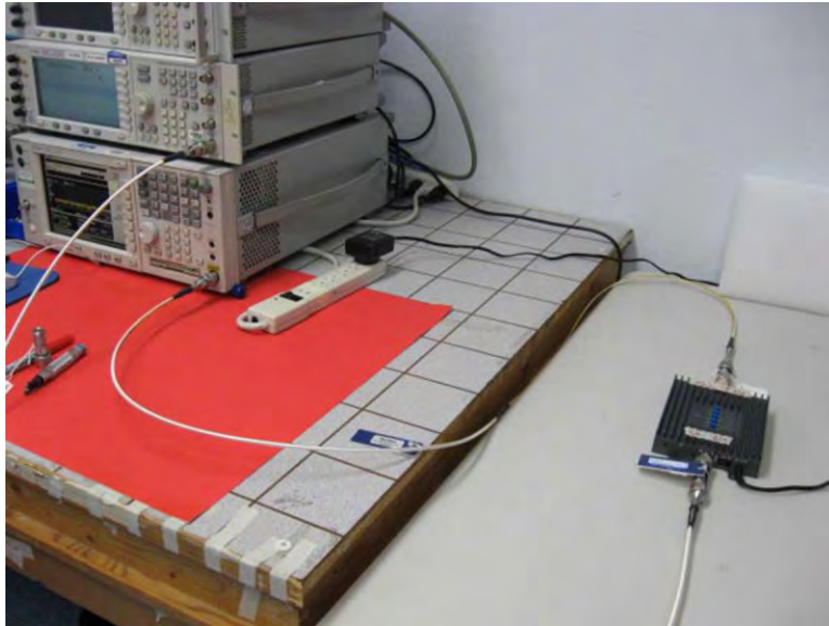
7.1, 7.2, 7.3, 7.5, 7.6 and 7.10 Test Setup
