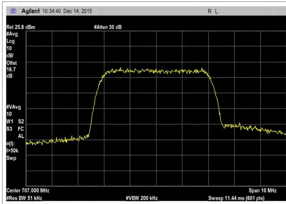
7.10_OBW_UL_698-716MHz_WCDMA
