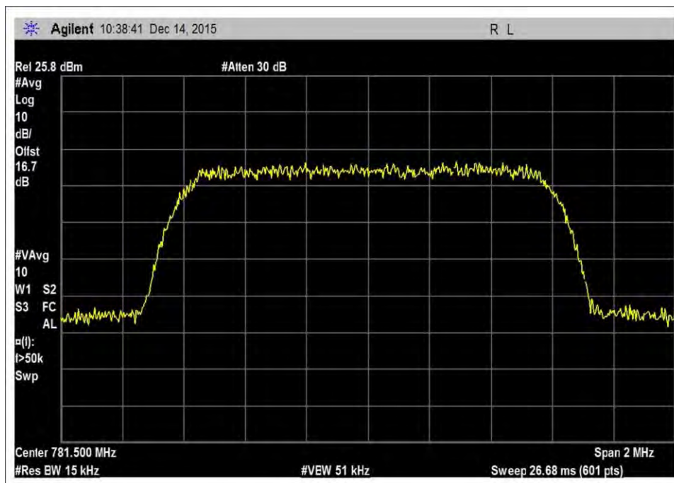
7.10_OBW_UL_776-787MHz_CDMA
