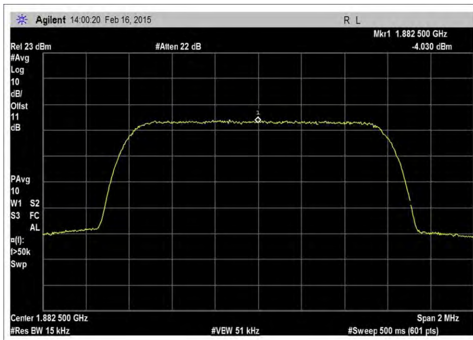
7.10_OBW_UL_1850-1915MHz_CDMA_Output
