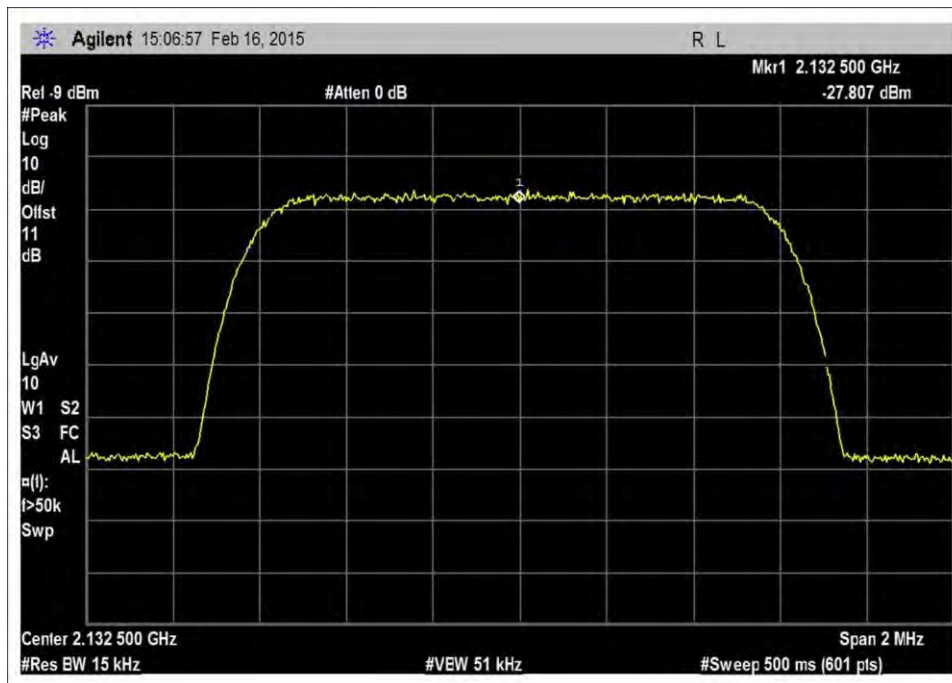
7.10_OBW_DL_2110-2155MHz_CDMA_Output
