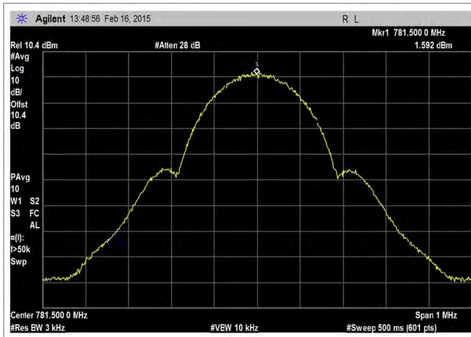
7.10_OBW_UL_776-787MHz_GSM_Output
