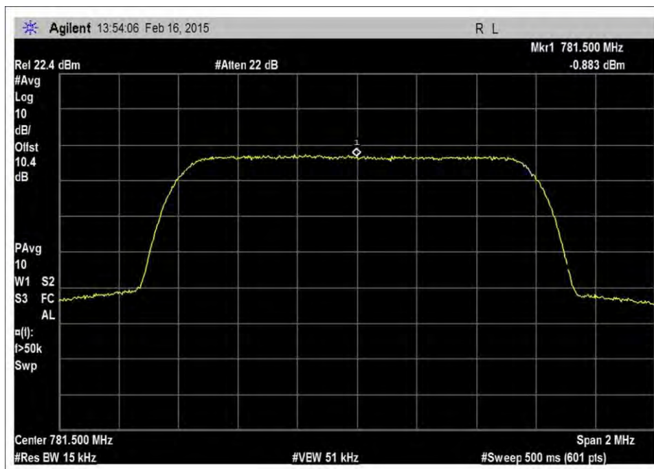
7.10_OBW_UL_776-787MHz_CDMA_Output
