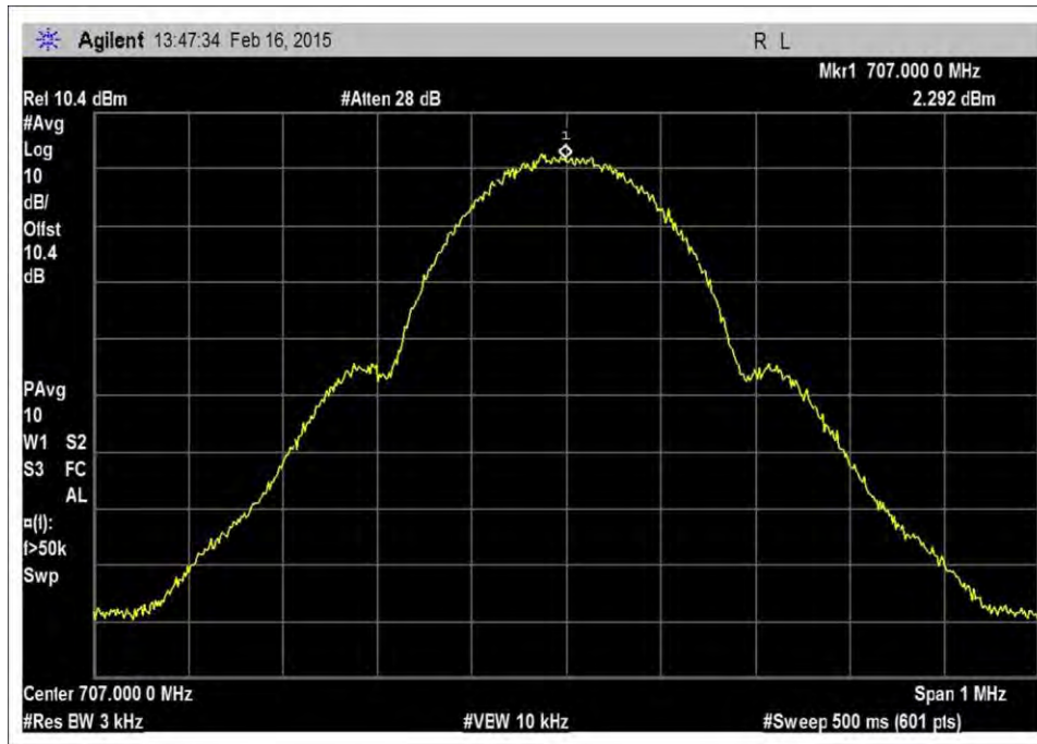
7.10_OBW_UL_698-716MHz_GSM_Output
