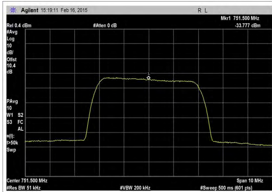
7.10_OBW_DL_746-757MHz_WCDMA_Output
