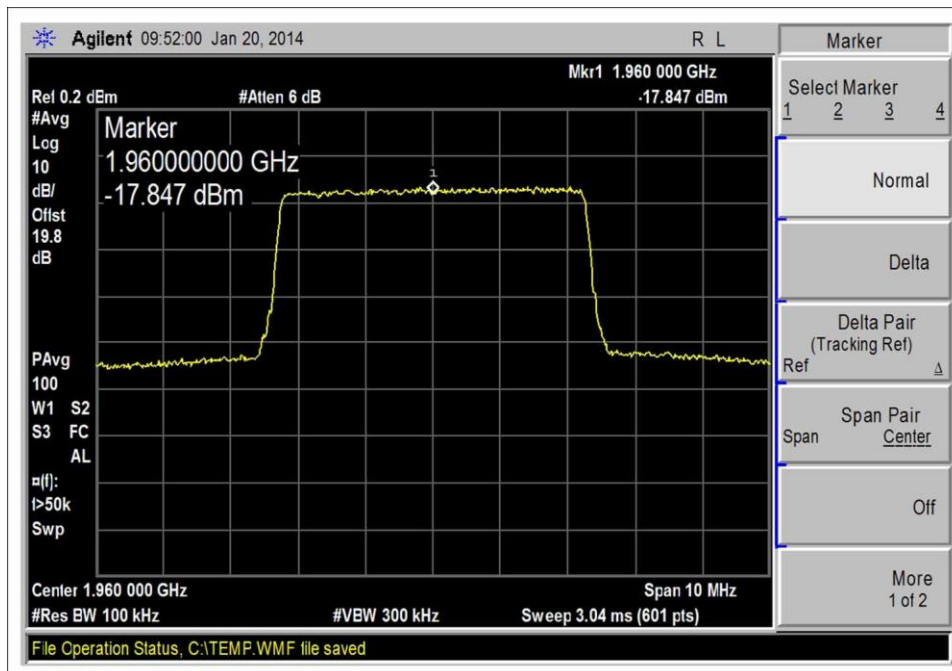
1930-1990MHz DL, LTE-Output
