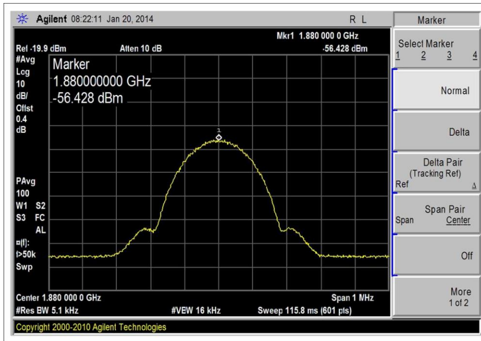
1850-1910MHz UL, GSM-Input
