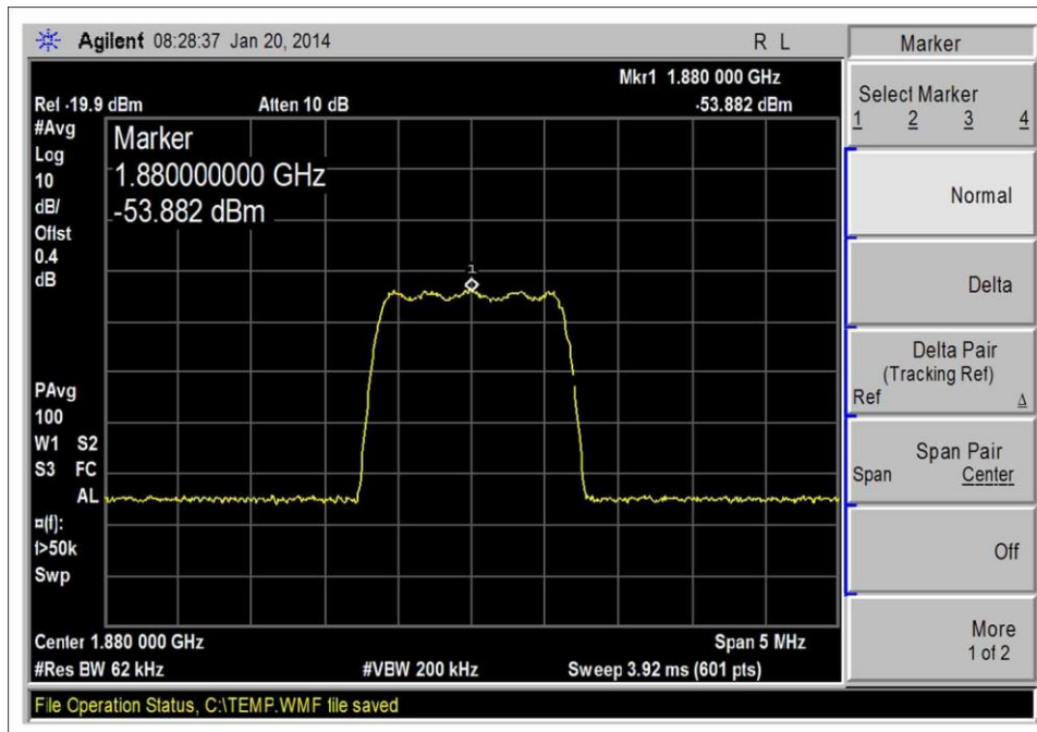
1850-1910MHz UL, CDMA-Input
