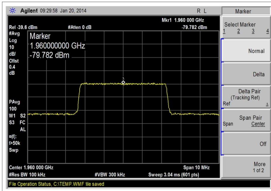
1930-1990MHz DL, LTE-Input
