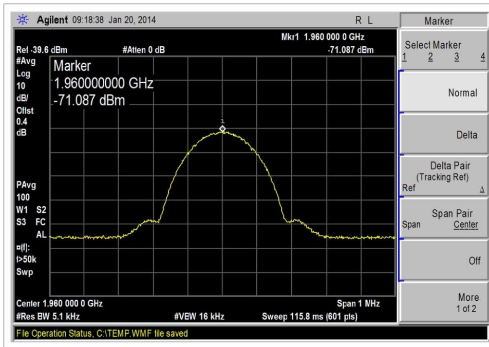
1930-1990MHz DL, GSM-Input
