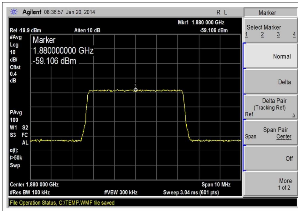
1850-1910MHz UL, LTE-Input
