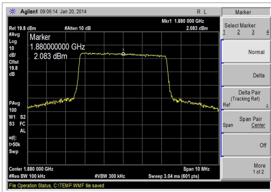
1850-1910MHz UL, LTE-Output
