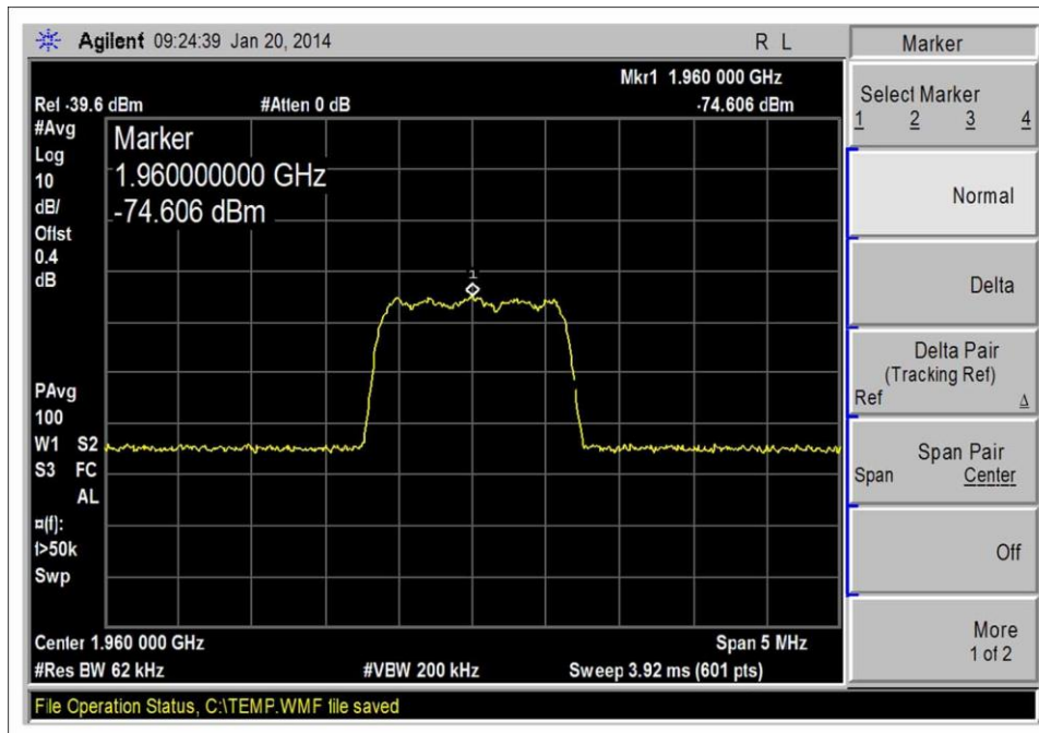
1930-1990MHz DL, CDMA-Input
