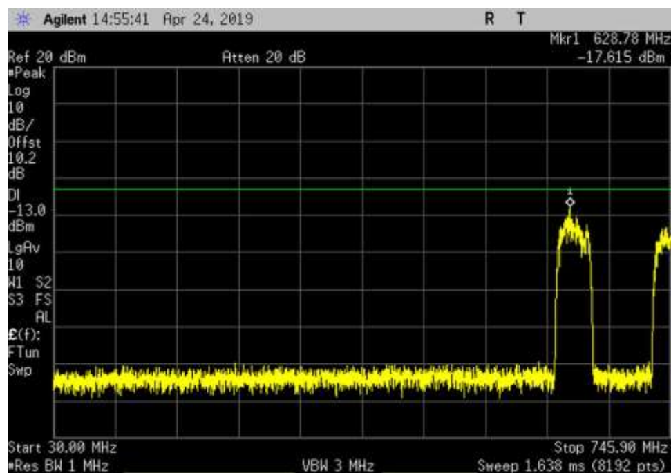
DL_746-757_GSM_30-745.9MHz_HC
