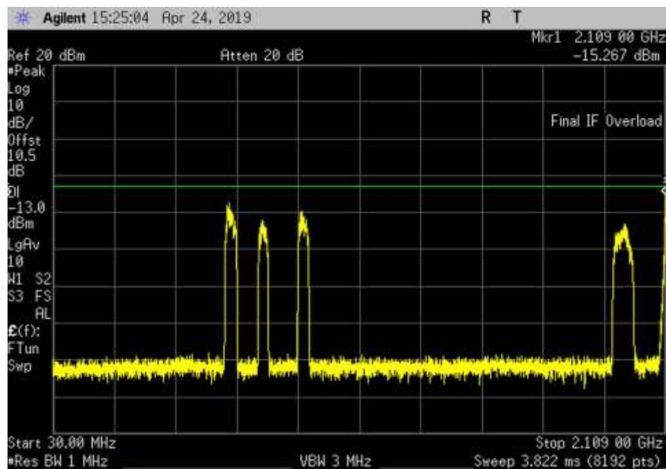
DL_2110-2155_AWGN_30-2109MHz_LC
