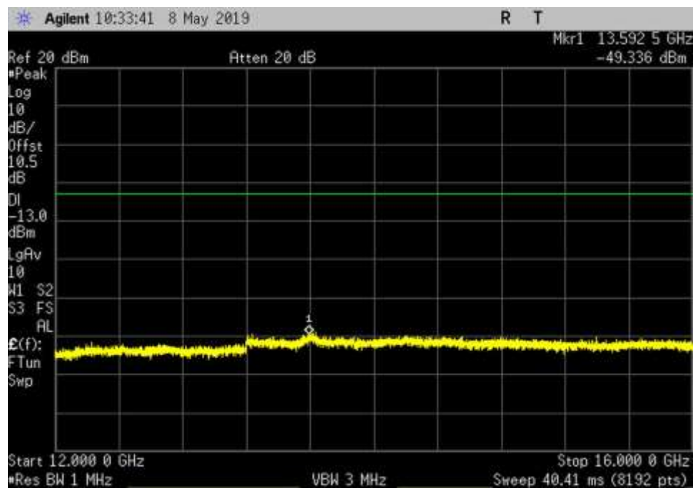
DL_2350-2360_AWGN_12000-16000MHz_MC
