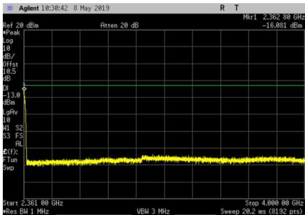
DL_2350-2360_AWGN_ 2361- 4000MHz_LC
