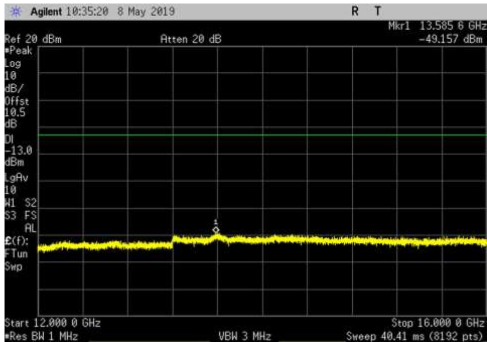
DL_2350-2360_AWGN_12000- 16000MHz_HC
