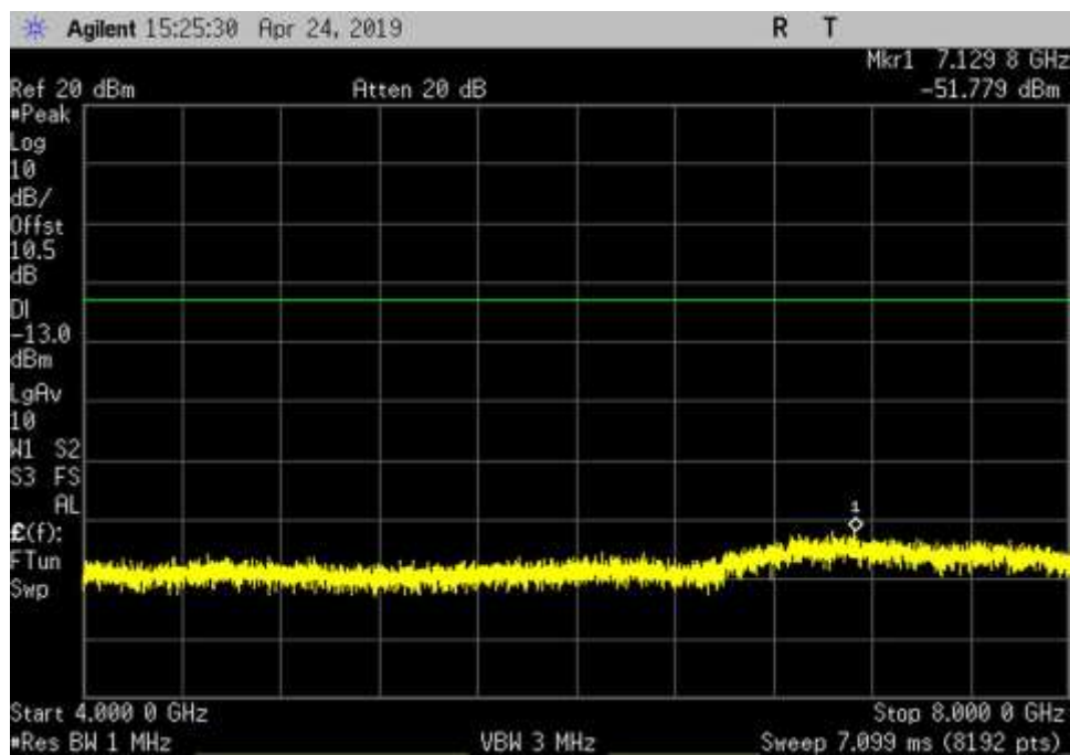
DL_2110-2155_AWGN_ 4000- 8000MHz_LC
