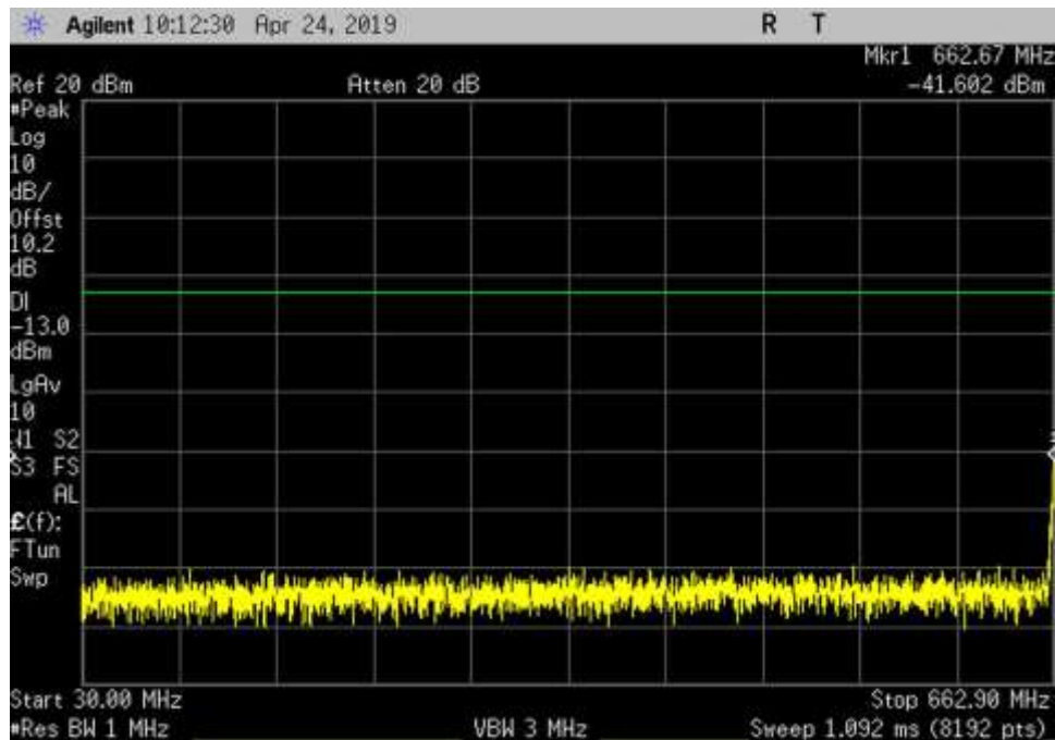
UL_663-698_GSM_30- 662.9MHz_MC
