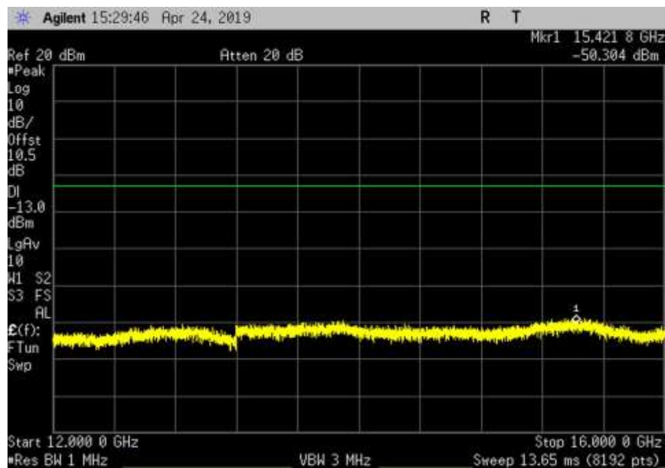
DL_2110-2155_AWGN_12000- 16000MHz_HC
