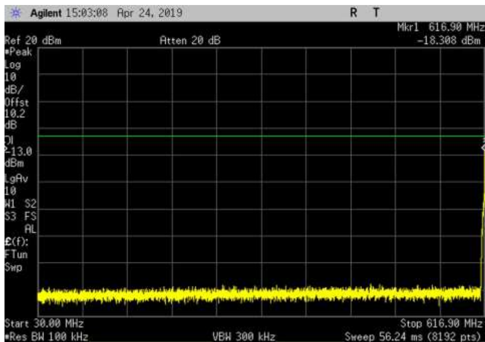
DL_617-652_GSM_30-616.9MHz_LC
