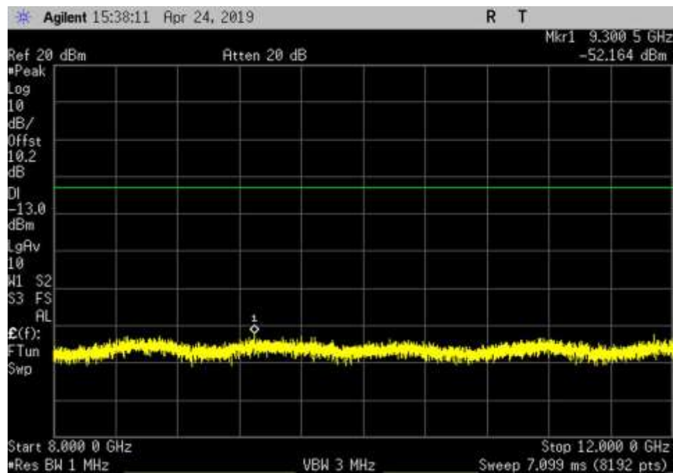
DL_869-894_AWGN_8000-12000MHz_LC
