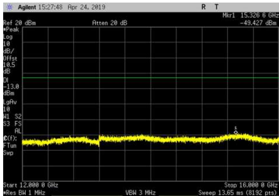
DL_2110-2155_AWGN_12000- 16000MHz_MC
