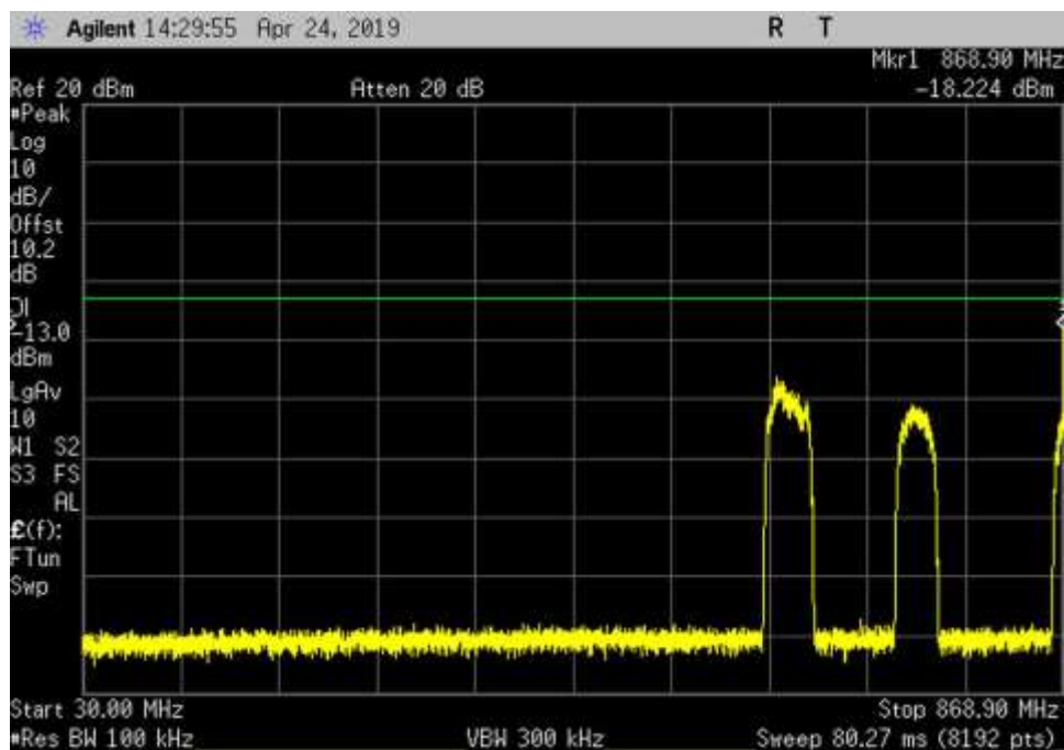
DL_869-894_GSM_30- 868.9MHz_LC
