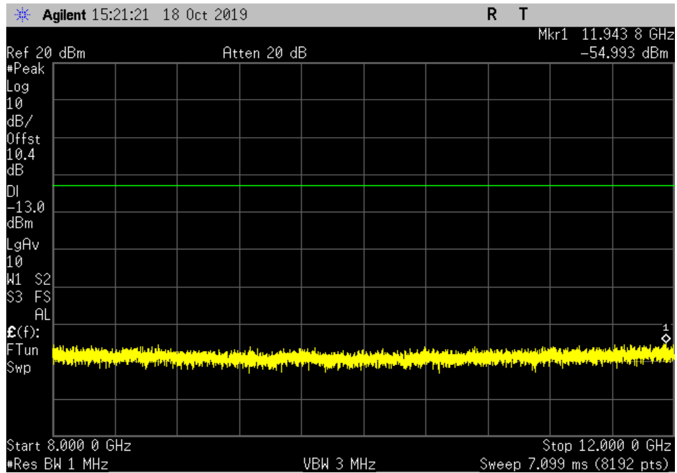
UL_1710-1755_GSM_8000-12000MHz_MC
