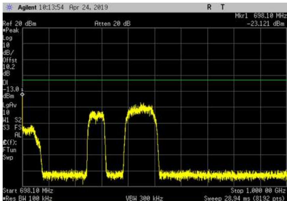
UL_663-698_GSM_698.1- 1000MHz_HC
