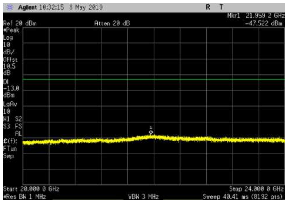
DL_2350-2360_AWGN_20000-24000MHz_LC
