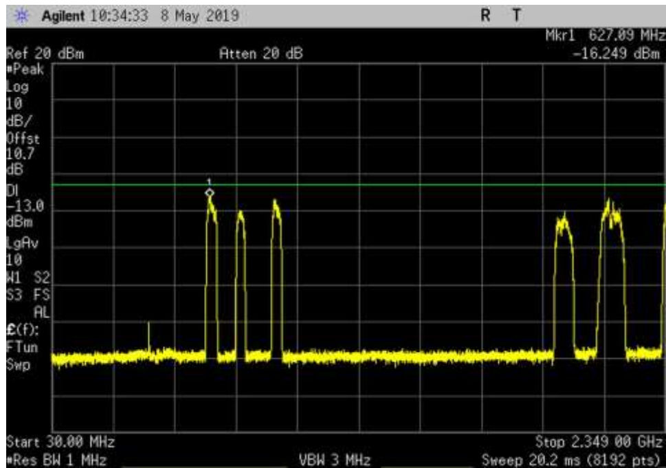
DL_2350-2360_AWGN_30- 2349MHz_HC
