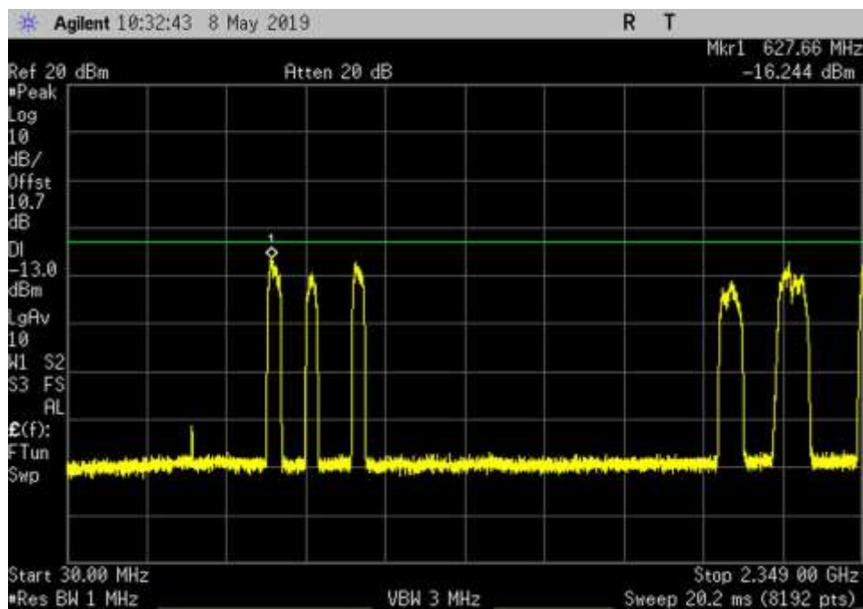
DL_2350-2360_AWGN_30- 2349MHz_MC
