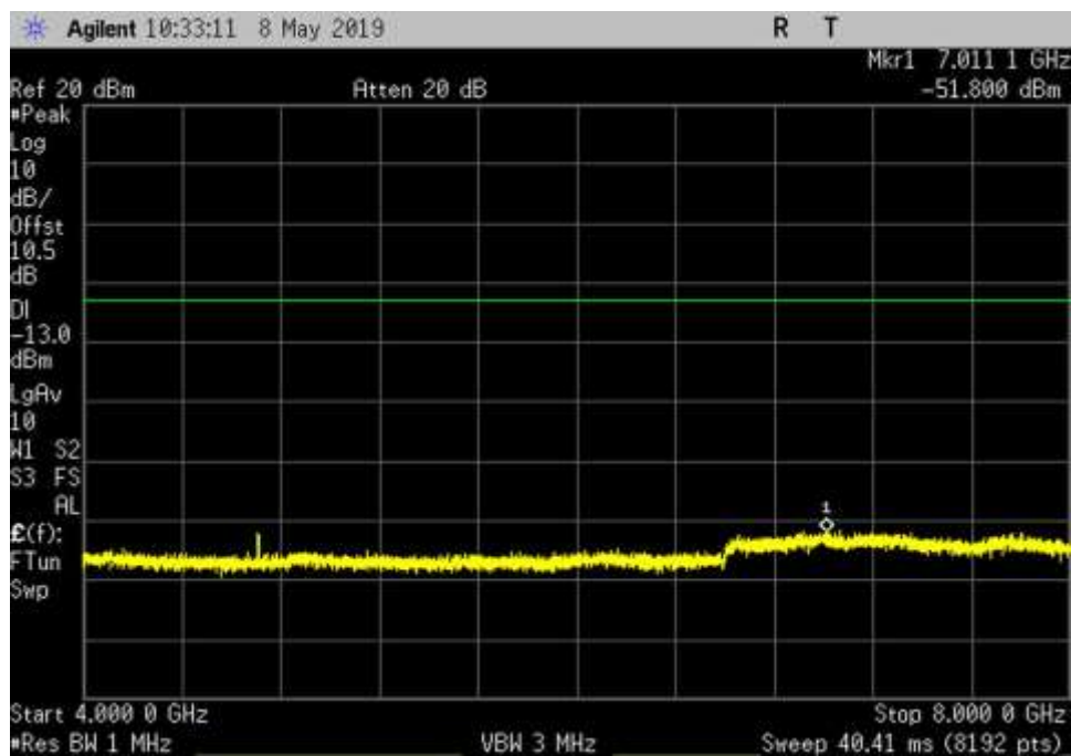
DL_2350-2360_AWGN_4000- 8000MHz_MC
