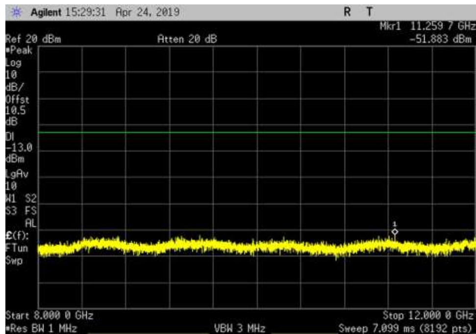
DL_2110-2155_AWGN_8000- 12000MHz_HC
