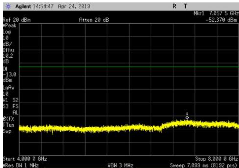
DL_746-757_GSM_4000-8000MHz_MC
