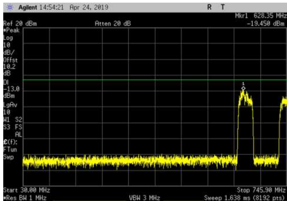
DL_746-757_GSM_30-745.9MHz_MC
