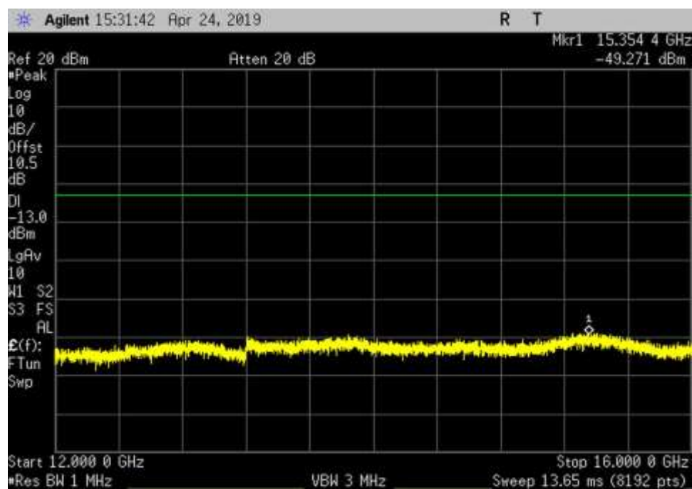
DL_1930-1995_AWGN_12000-16000MHz_LC
