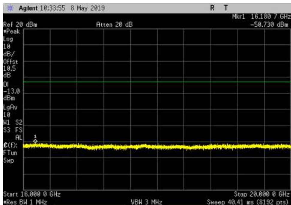
DL_2350-2360_AWGN_16000-20000MHz_MC
