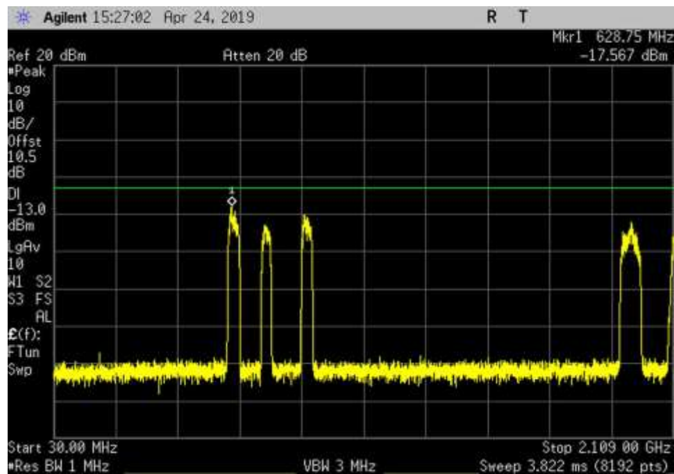
DL_2110-2155_AWGN_30- 2109MHz_MC
