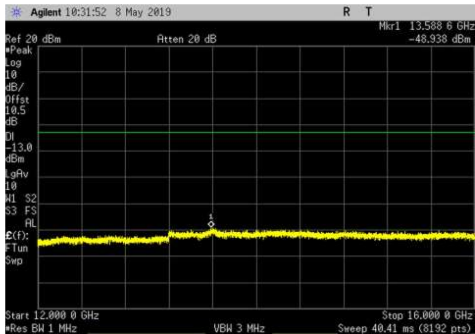
DL_2350-2360_AWGN_12000-16000MHz_LC
