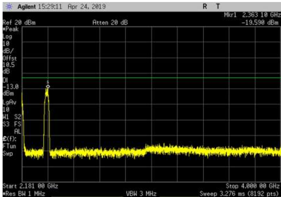
CSE_DL_2110-2155_AWGN_ 2181- 4000MHz_HC
