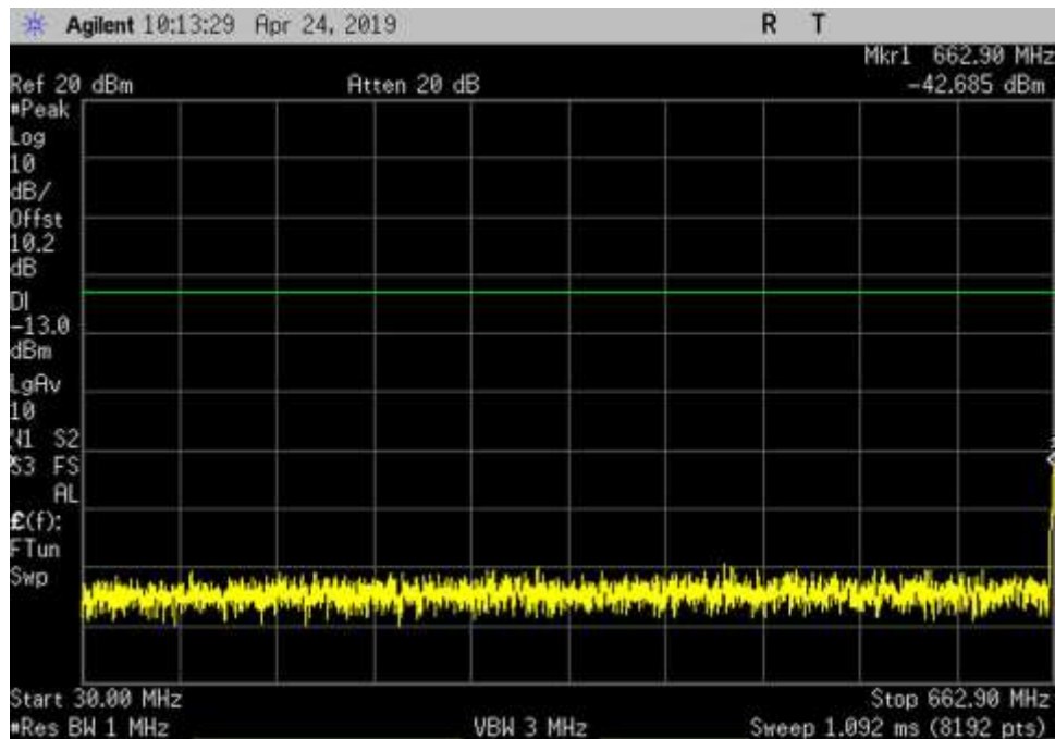
UL_663-698_GSM_30- 662.9MHz_HC
