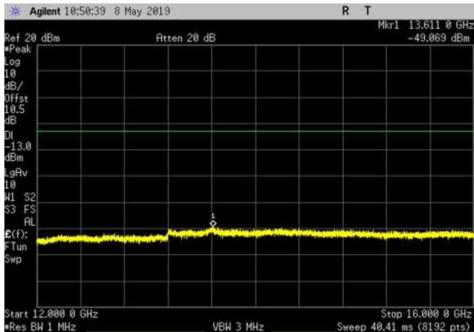
UL_2305-2315_GSM_12000- 16000MHz_LC
