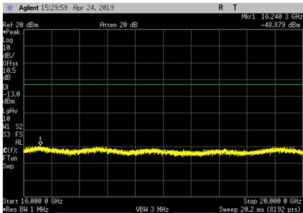
DL_2110-2155_AWGN_16000- 20000MHz_HC
