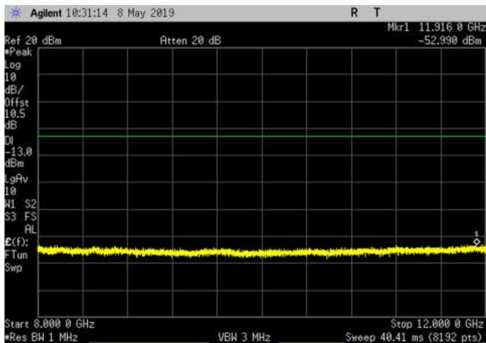
DL_2350-2360_AWGN_8000- 12000MHz_LC
