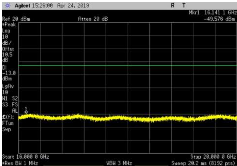
DL_2110-2155_AWGN_16000-20000MHz_LC
