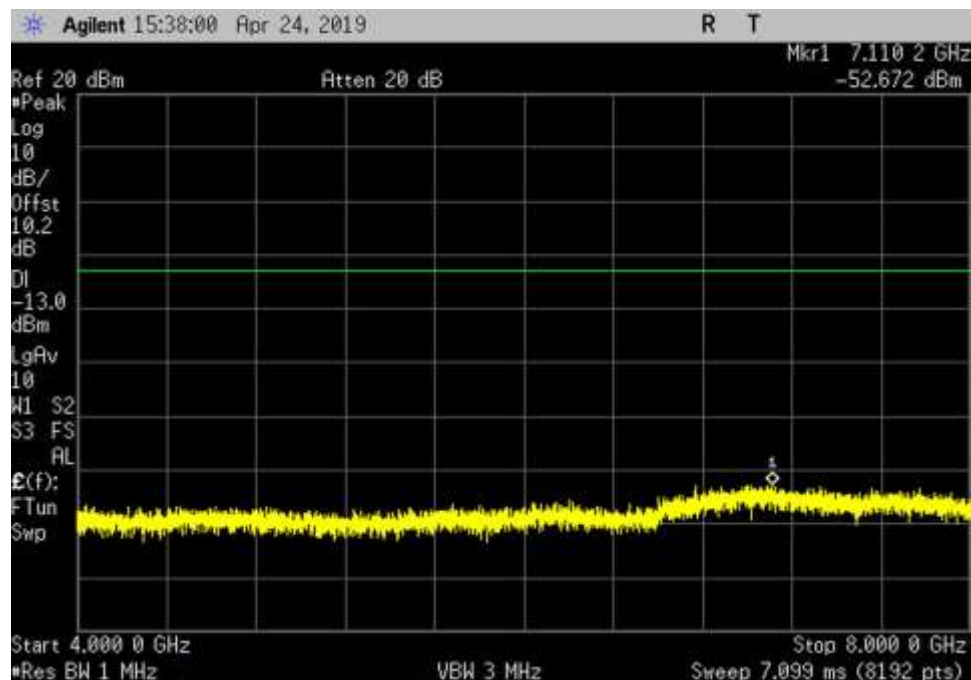
DL_869-894_AWGN_4000-8000MHz_LC
