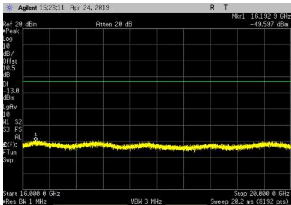
DL_2110-2155_AWGN_16000-20000MHz_MC
