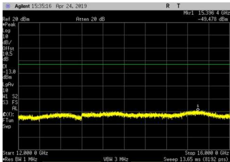
DL_1930-1995_AWGN_12000- 16000MHz_HC
