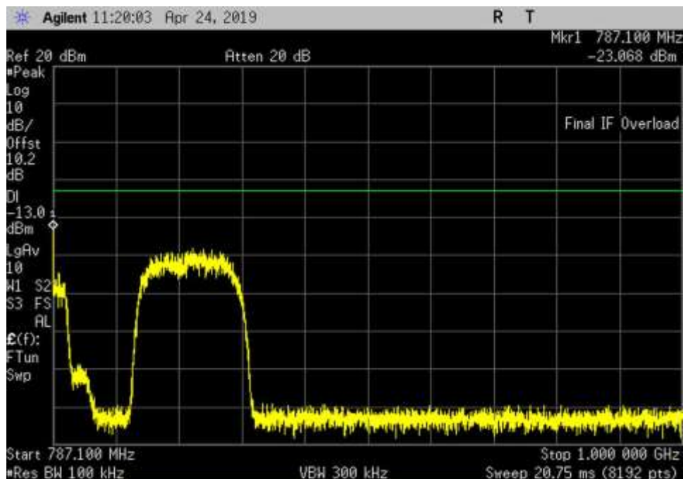
UL_776-787_GSM_787.1-1000MHz_HC
