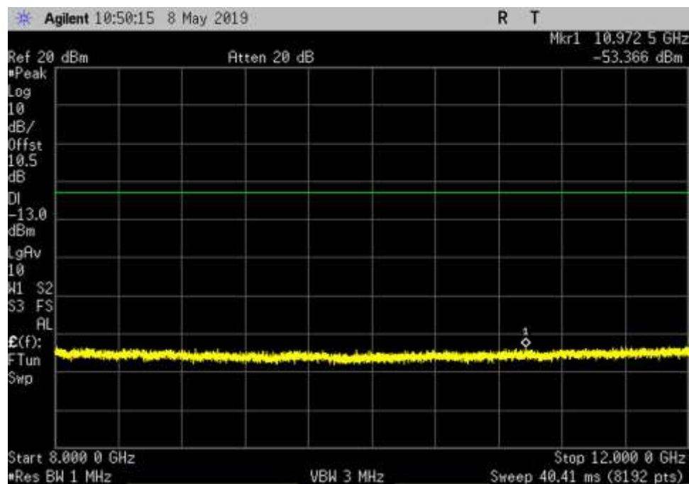
UL_2305-2315_GSM_8000-12000MHz_LC
