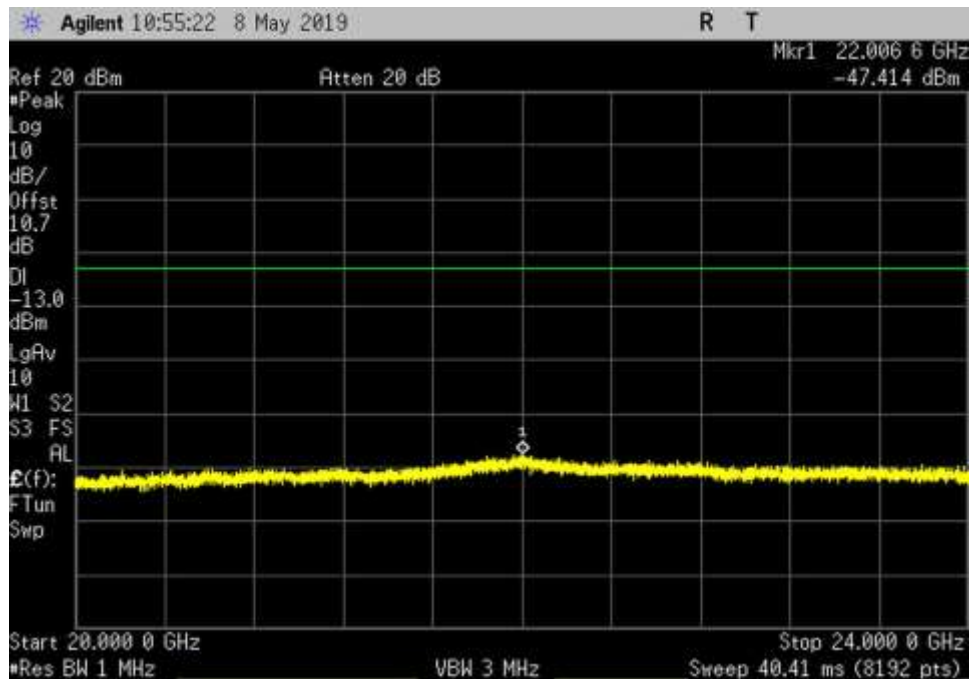
UL_2305-2315_GSM_20000-24000MHz_HC
