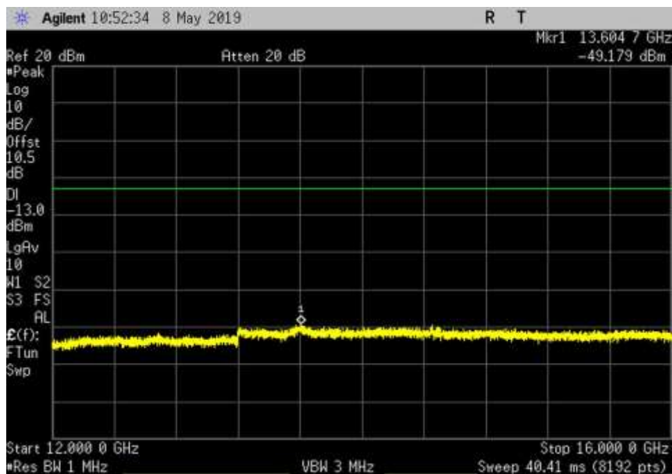
UL_2305-2315_GSM_12000- 16000MHz_MC
