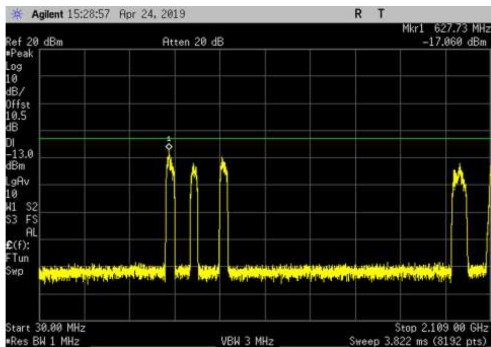
DL_2110-2155_AWGN_30- 2109MHz_HC
