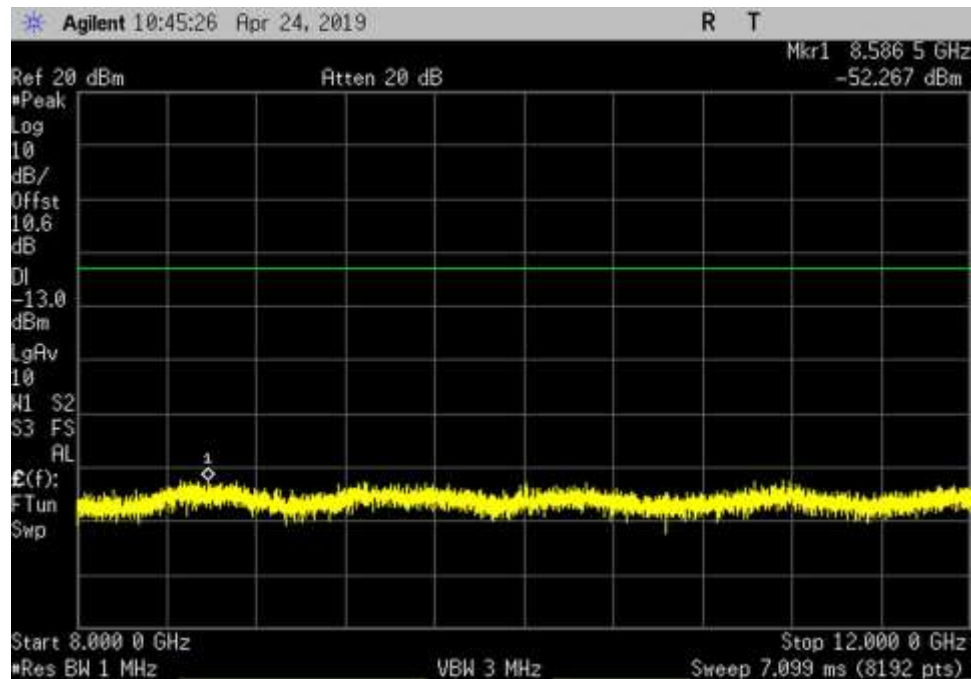
UL_1850-1915_GSM_8000-12000MHz_MC
