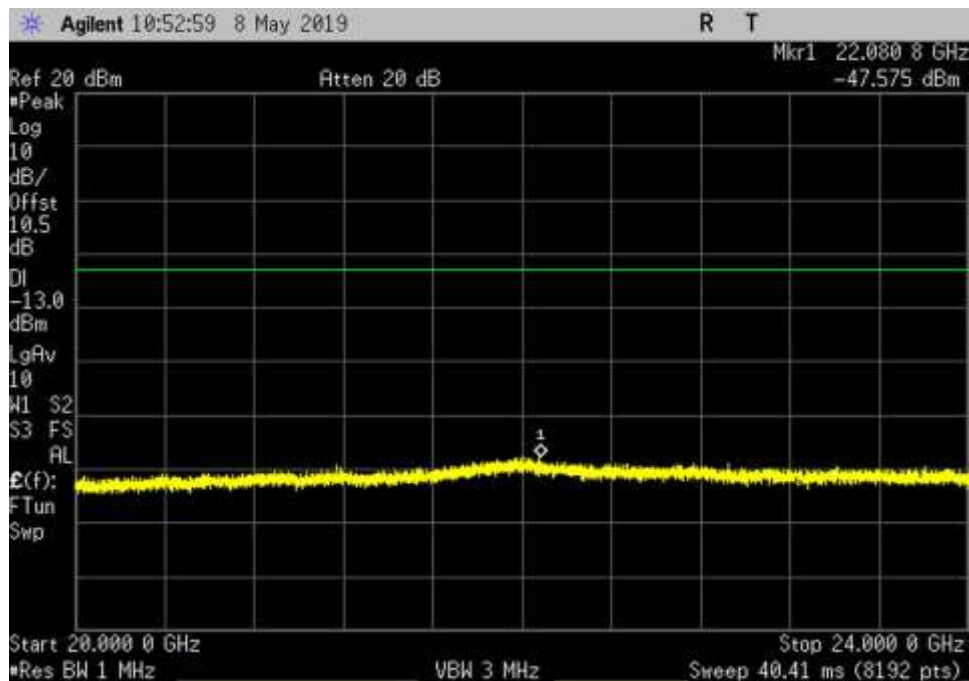
3.6.3 CSE_UL_2305-2315_GSM_20000-24000MHz_MC
