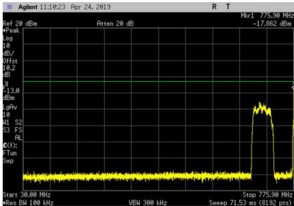
UL_776-787_GSM_30- 775.9MHz_LC
