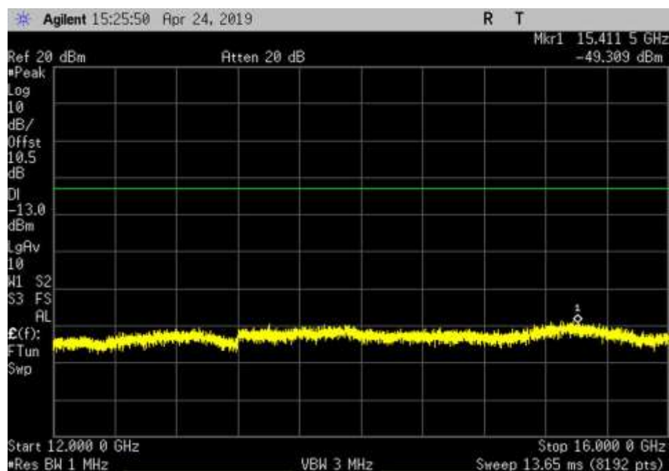
DL_2110-2155_AWGN_12000- 16000MHz_LC
