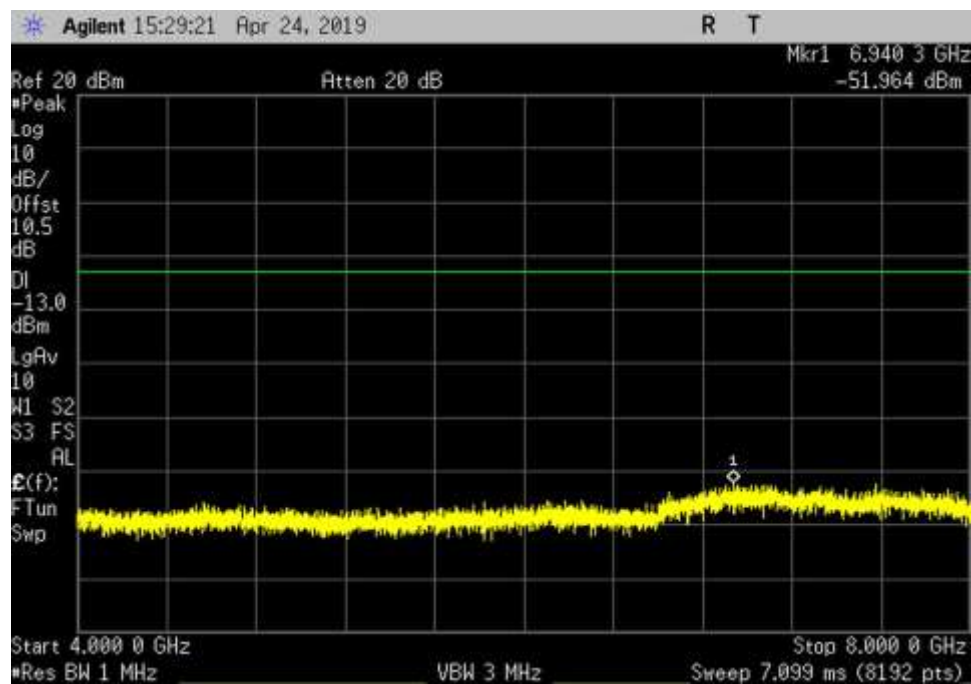
DL_2110-2155_AWGN_ 4000- 8000MHz_HC
