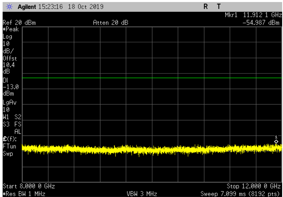
UL_1710-1755_GSM_8000-12000MHz_HC
