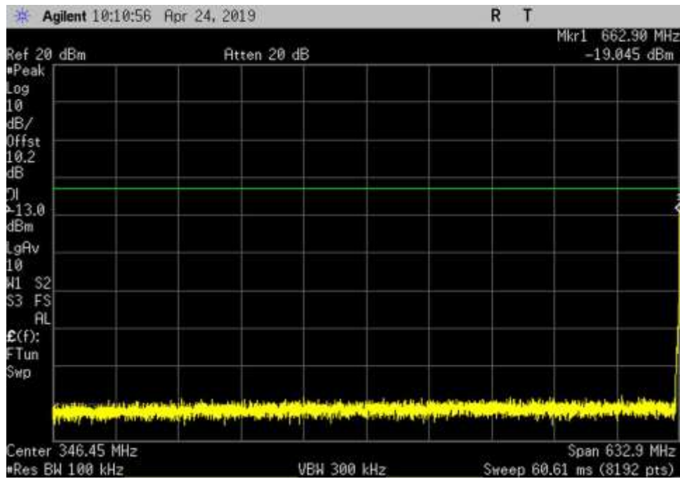
UL_663-698_GSM_30- 662.9MHz_LC
