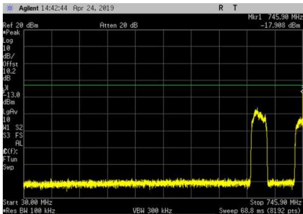
DL_746-757_GSM_30- 745.9MHz_LC
