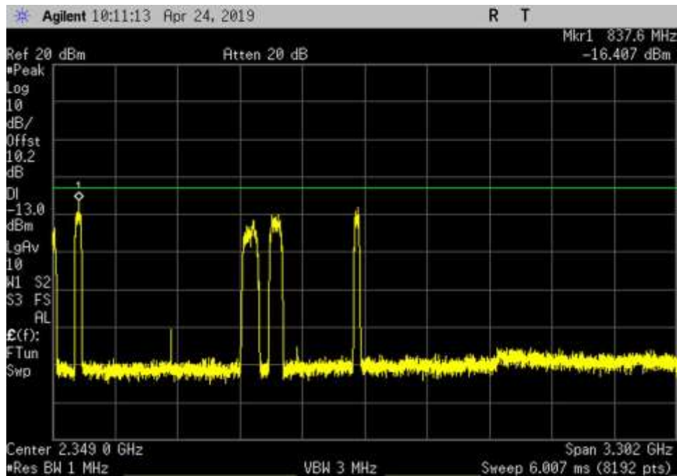
UL_663-698_GSM_698.1- 4000MHz_LC
