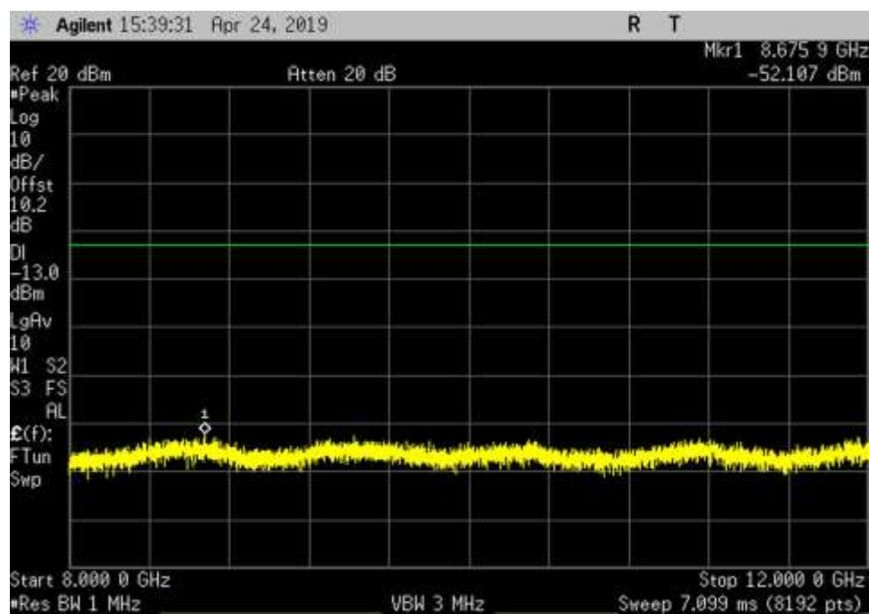
DL_869-894_AWGN_8000-12000MHz_MC
