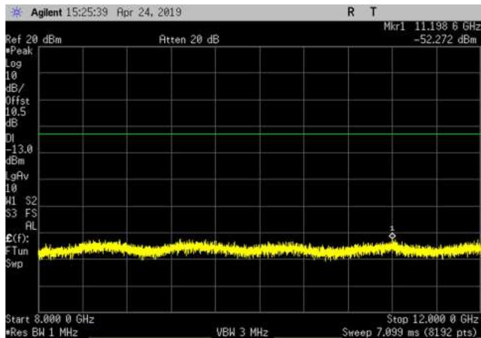
DL_2110-2155_AWGN_8000- 12000MHz_LC
