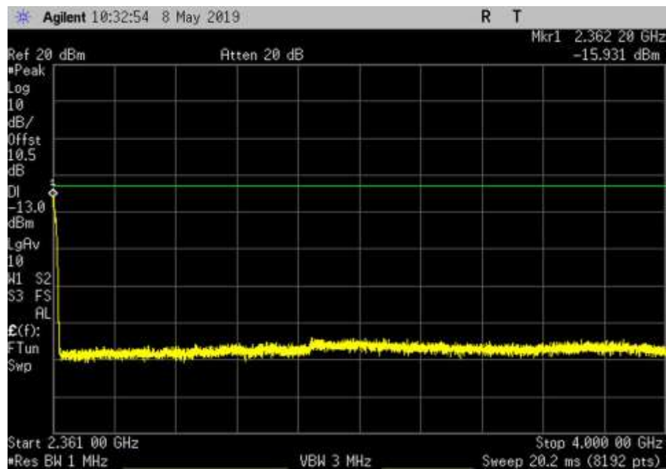
DL_2350-2360_AWGN_2361- 4000MHz_MC
