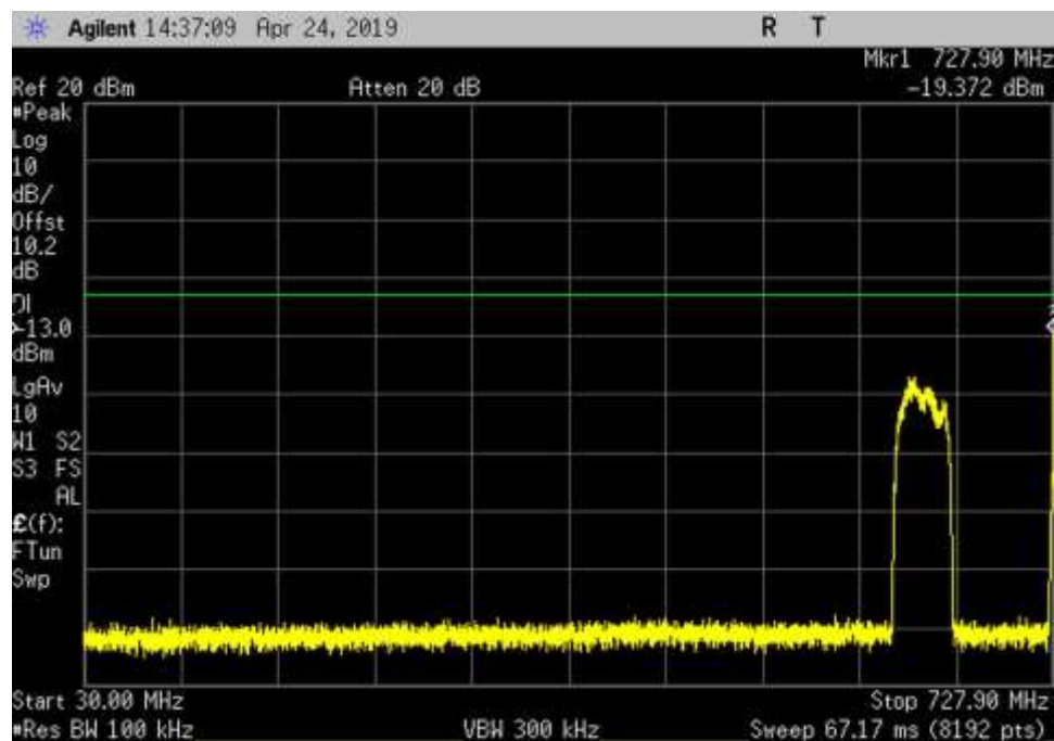
DL_728-746_GSM_30- 727.9MHz_LC
