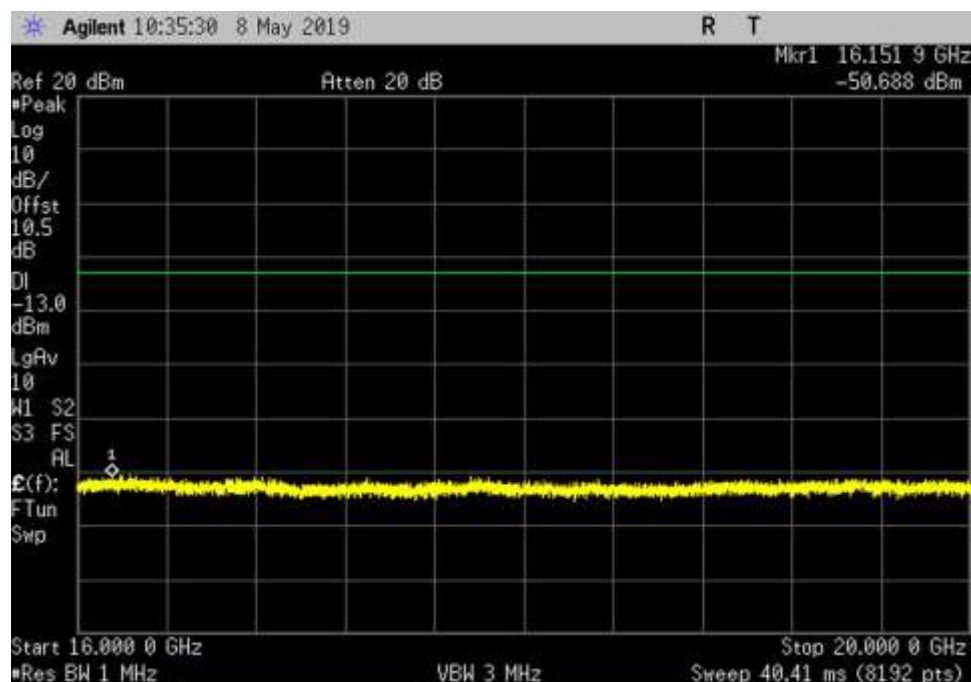
DL_2350-2360_AWGN_16000-20000MHz_HC
