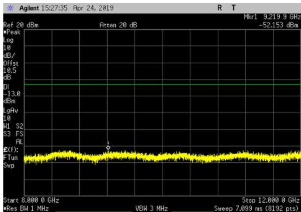
DL_2110-2155_AWGN_8000- 12000MHz_MC
