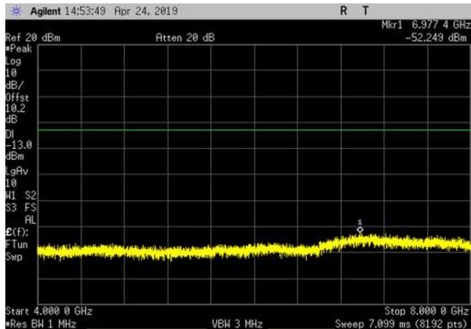
DL_746-757_GSM_4000-8000MHz_LC
