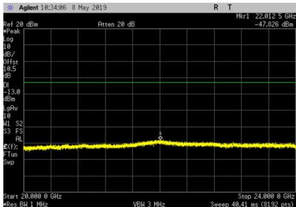
DL_2350-2360_AWGN_20000-24000MHz_MC
