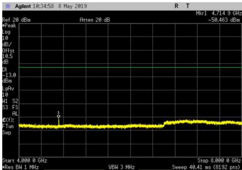
DL_2350-2360_AWGN_4000- 8000MHz_HC
