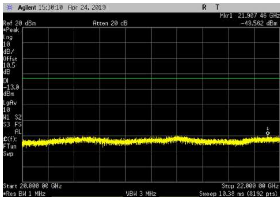
DL_2110-2155_AWGN_20000-22000MHz_HC
