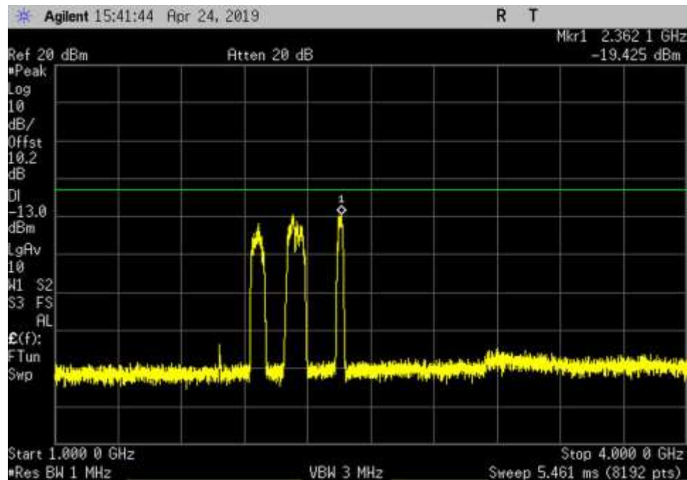
DL_869-894_AWGN_1000-4000MHz_HC
