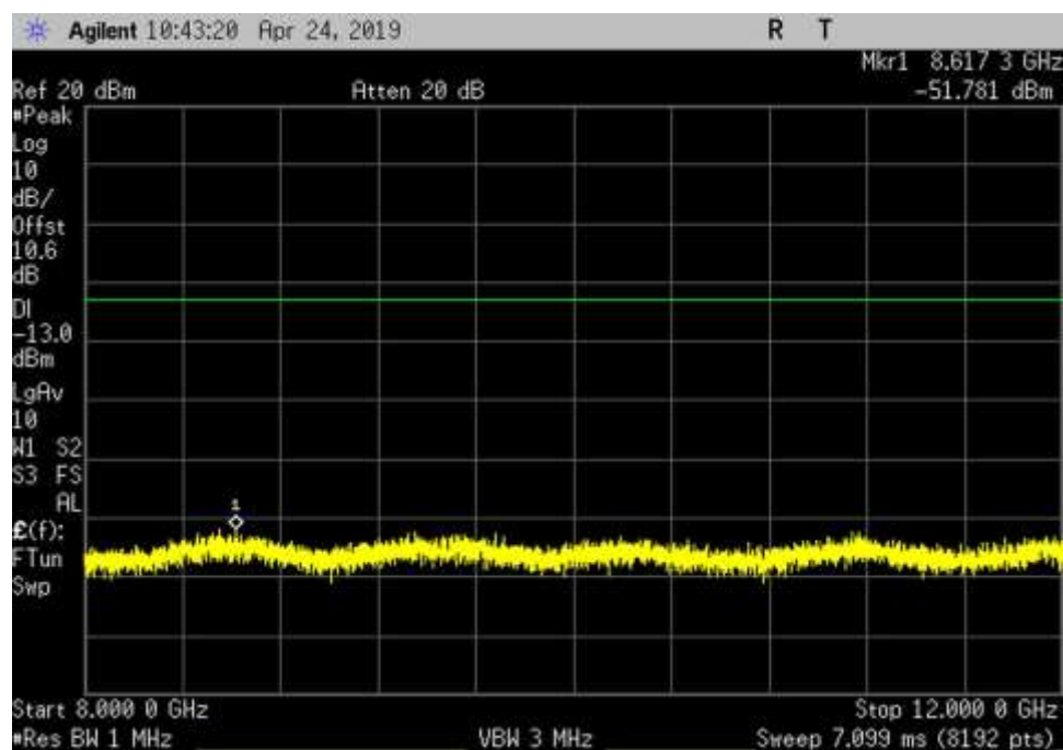
UL_1850-1915_GSM_8000-12000MHz_LC
