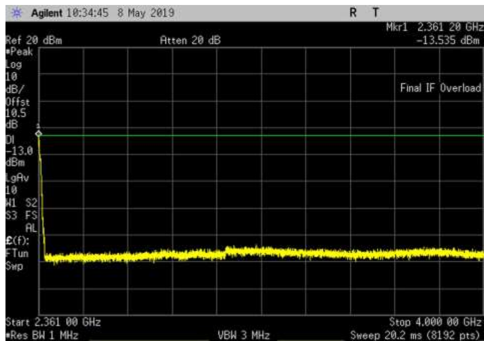
DL_2350-2360_AWGN_2361- 4000MHz_HC
