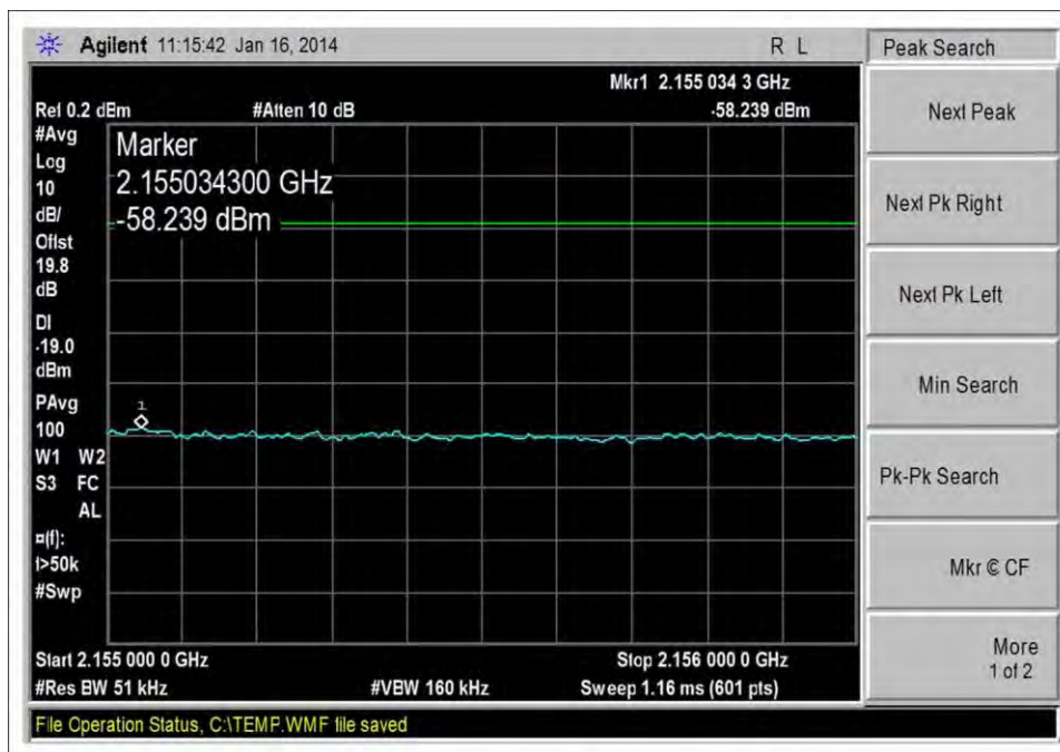
DL_2110-2155MHz_CDMA_H_-62dBm
