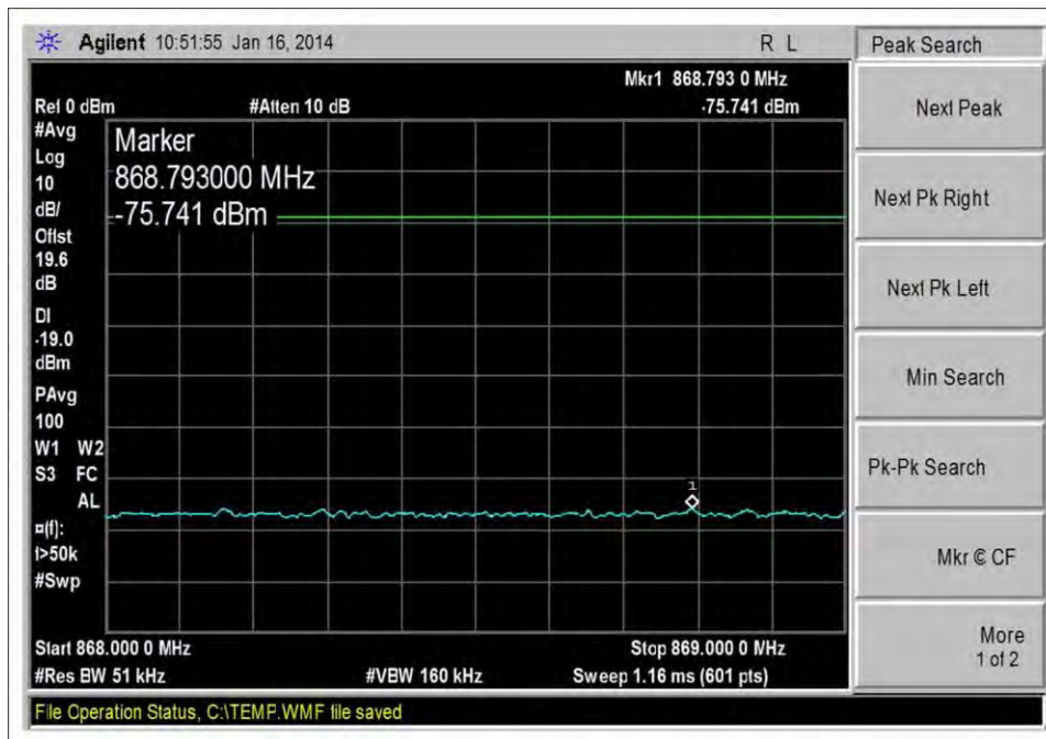
DL_869-880MHz_CDMA_L_-20dBm
