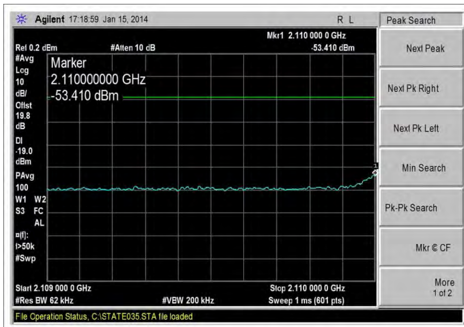
DL_2110-2155MHz_LTE_L_-62dBm
