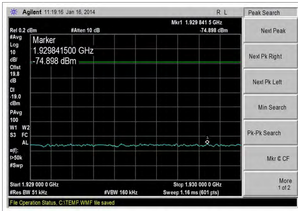
DL_1930-1995MHz_CDMA_L_-20dBm
