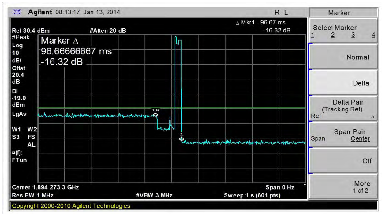
Uplink 1850-1915MHz Oscillation Detection Screen Capture
