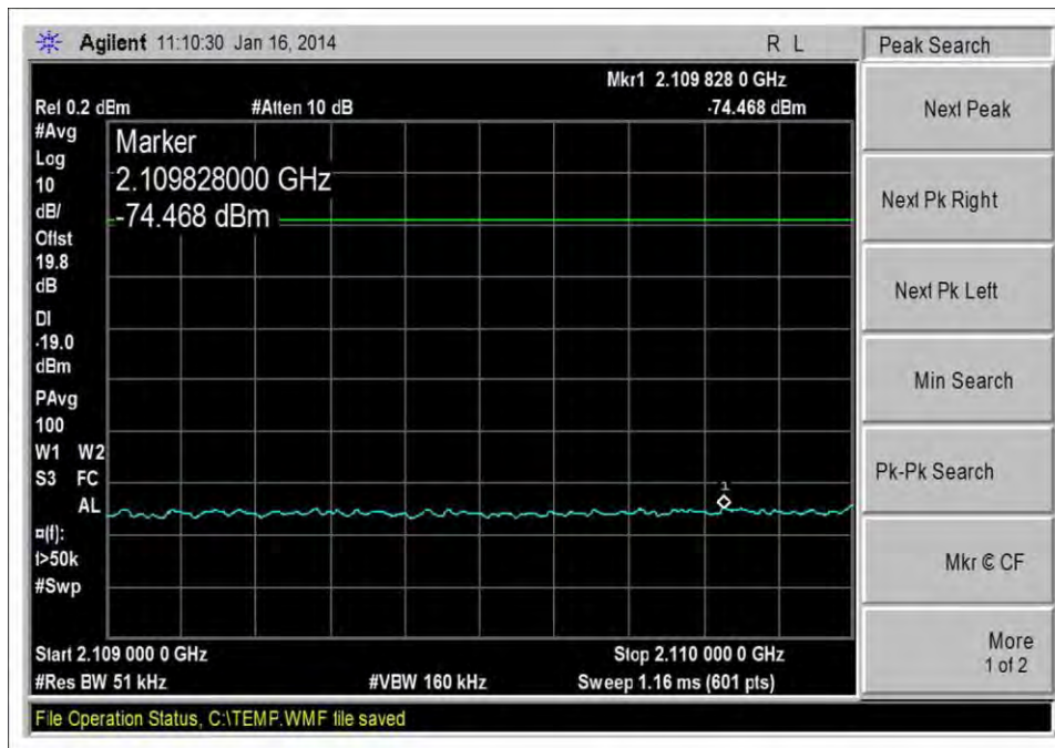
7.5_OBE_DL_2110-2155MHz_CDMA_L_-20dBm
