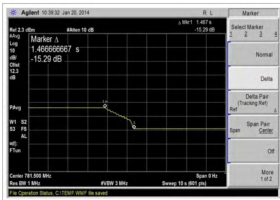
VariableNoiseTiming_UL_776-787MHz
