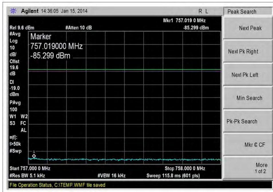
DL_746-757MHz_GSM_H_-20dBm
