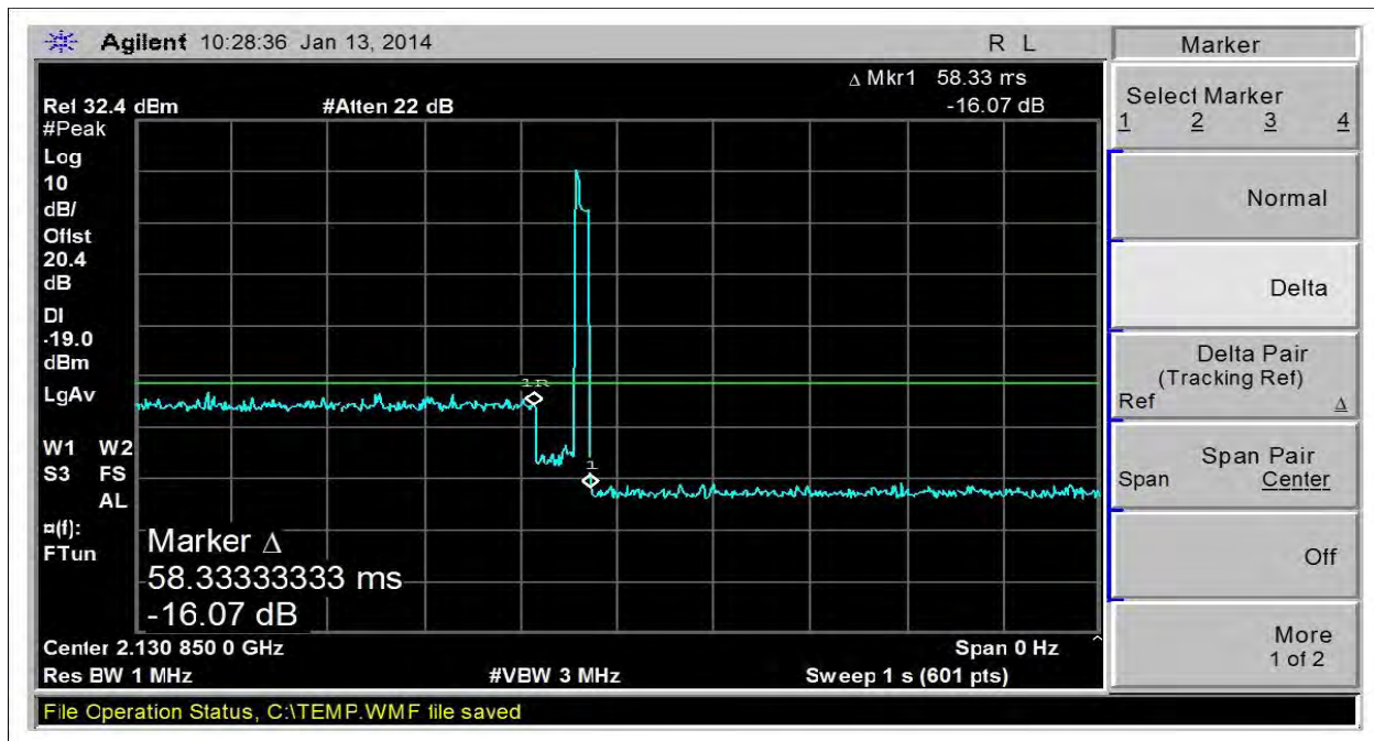
Downlink 2110-2155MHz Oscillation Detection Screen Capture
