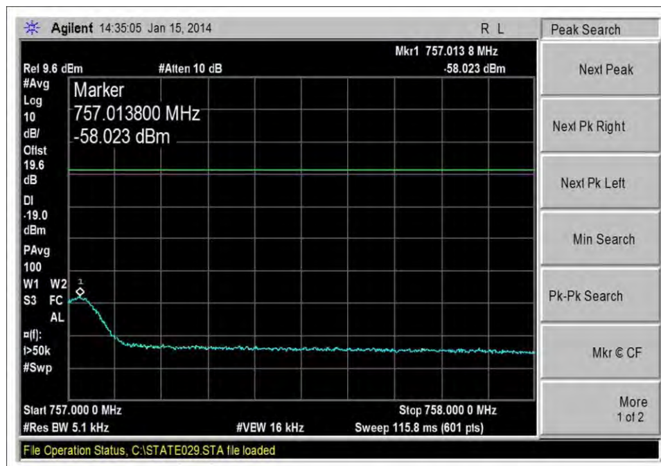
DL_746-757MHz_GSM_H_-63dBm
