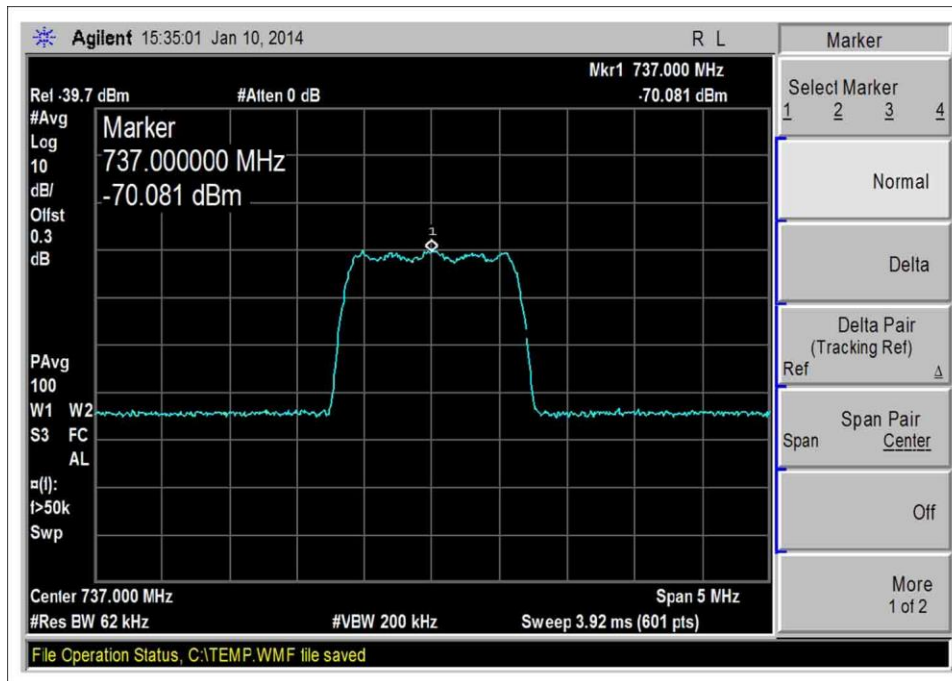
728-746MHz DL, CDMA-Input
