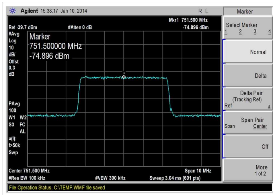
746-757MHz DL, LTE-Input
