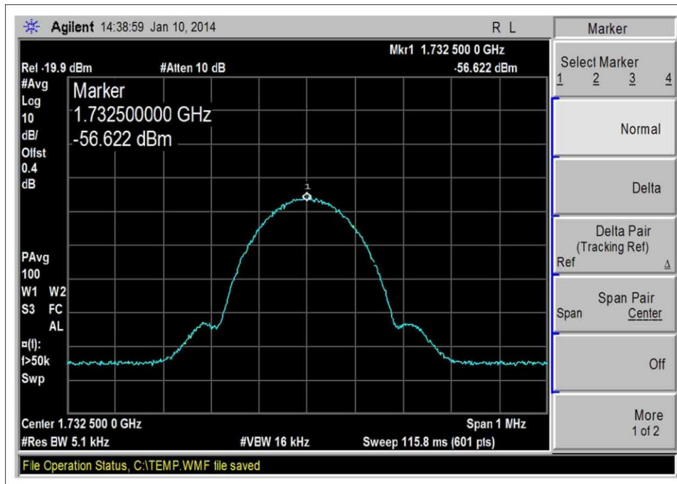
1710-1755 UL, GSM-Input
