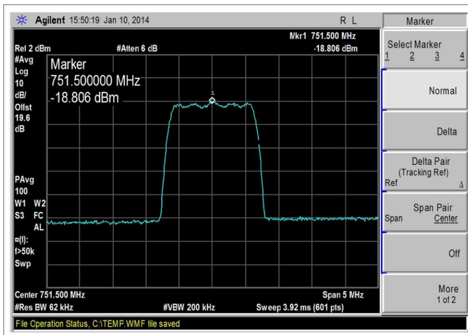
746-757MHz DL, CDMA-Output
