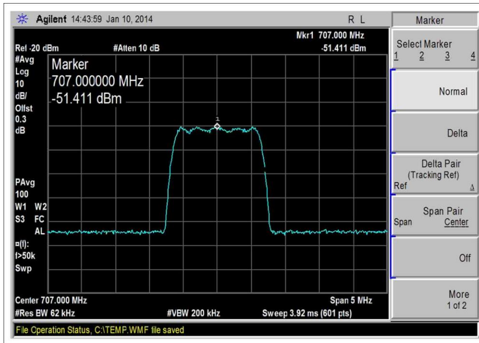
698-716MHz UL, CDMA-Input
