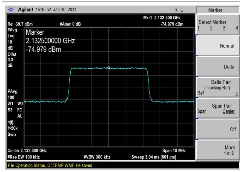
2110-2135MHz DL, LTE-Input
