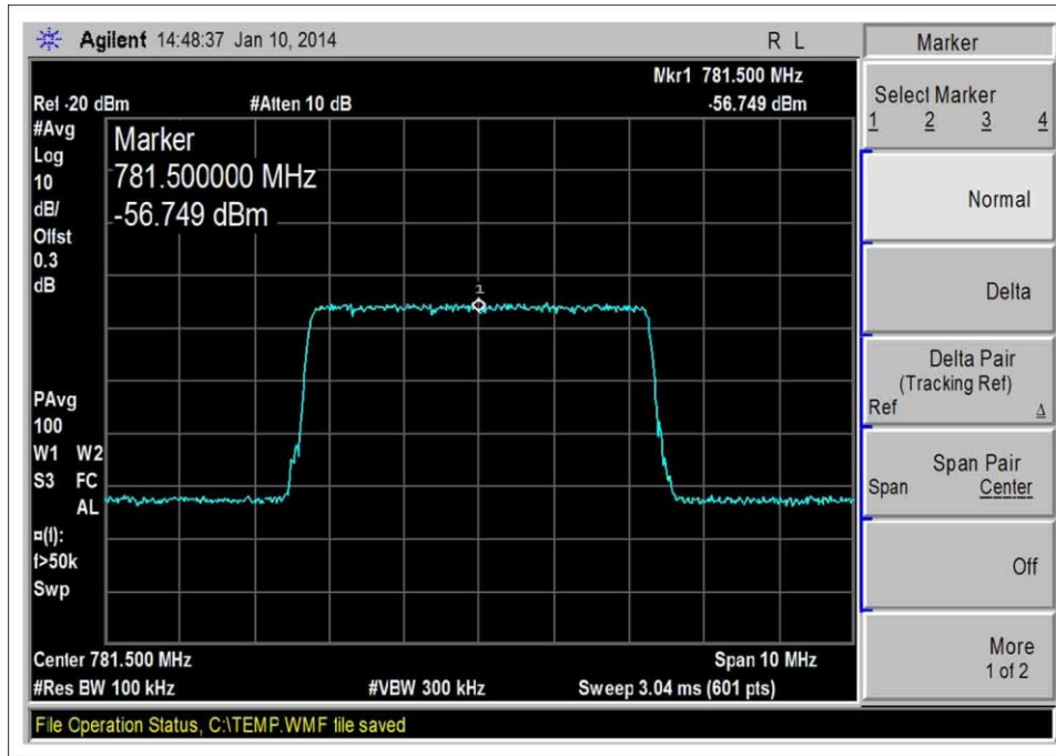
776-787MHz UL, LTE-Input
