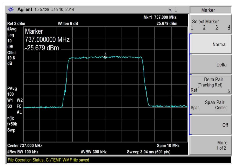
728-746MHz DL, LTE-Output
