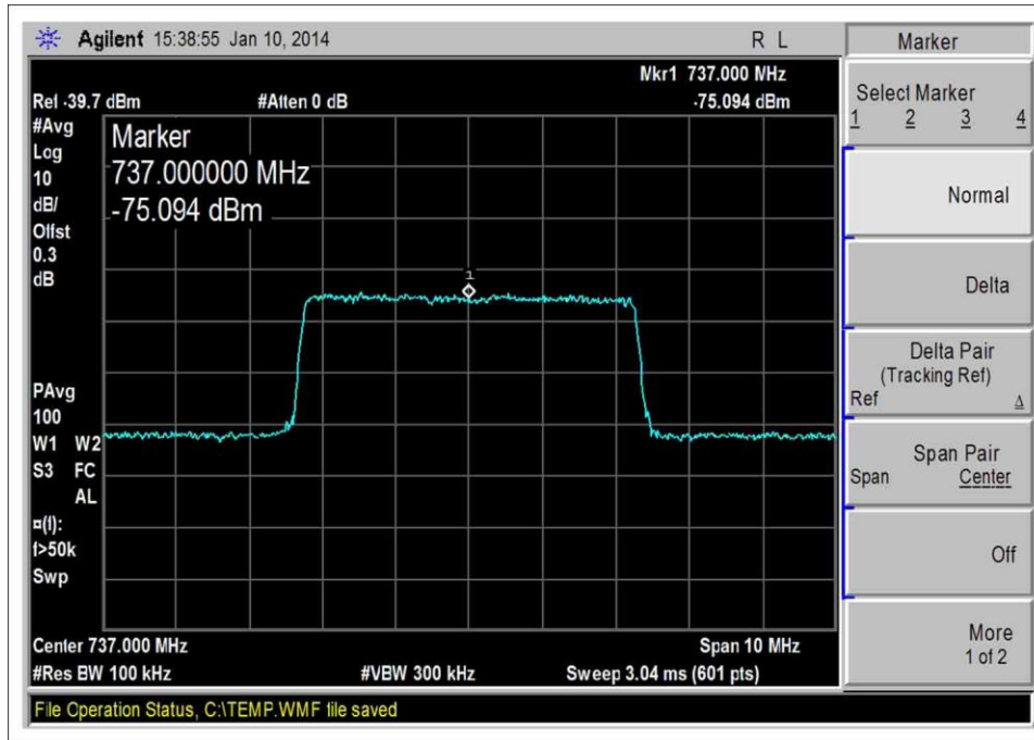
728-746MHz DL, LTE-Input
