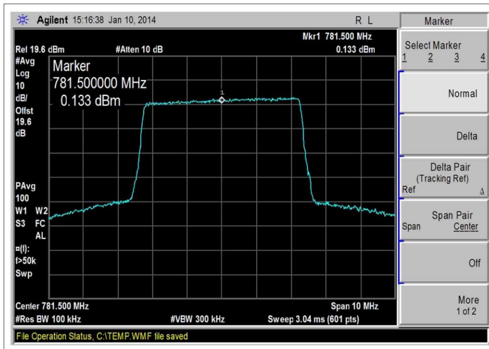
776-787MHz UL, LTE-Output
