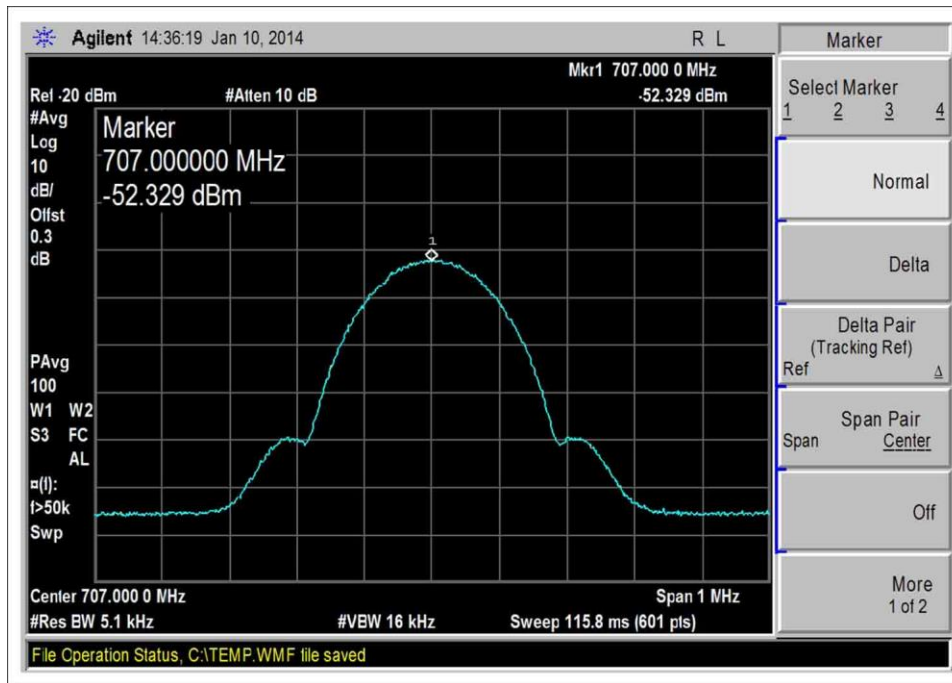
698-716MHz UL, GSM-Input
