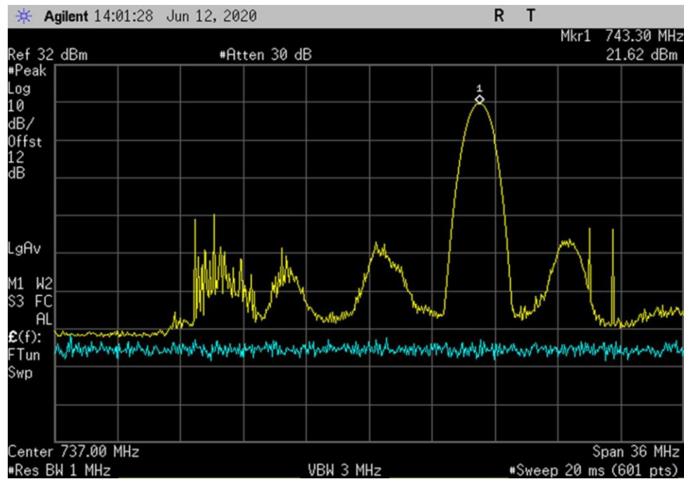
DL_728-746_Pk_737MHz
