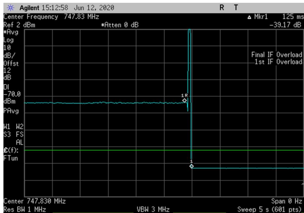
DL_746-757_747.83MHz
