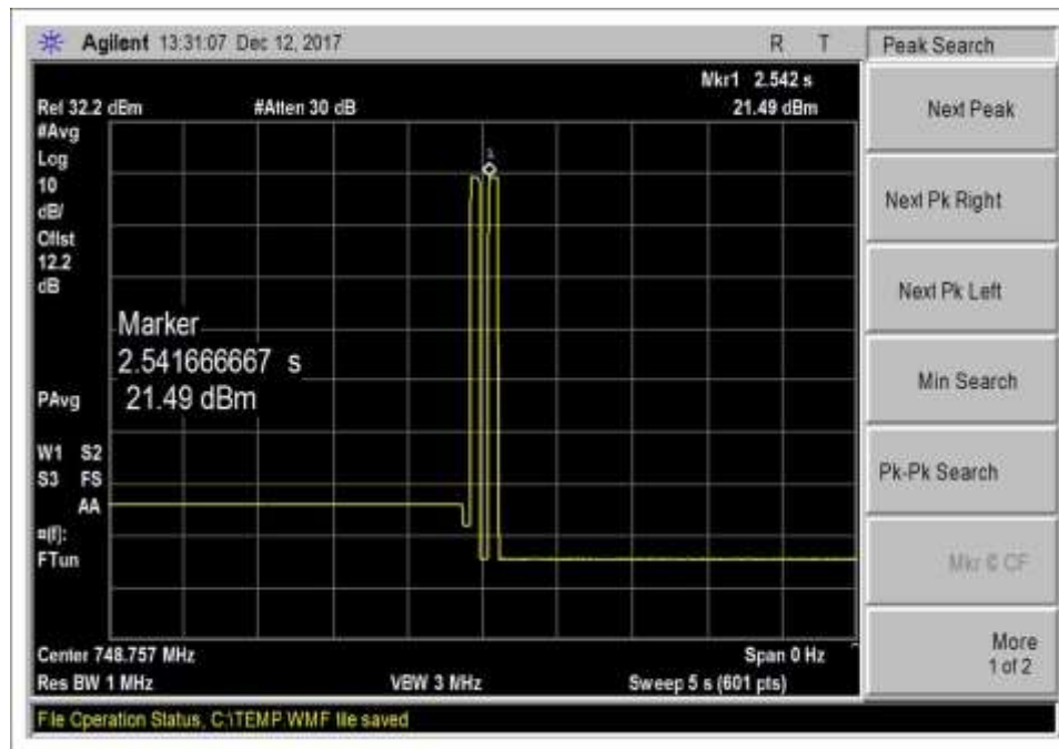
7.11.2 DL 746-757 peak
