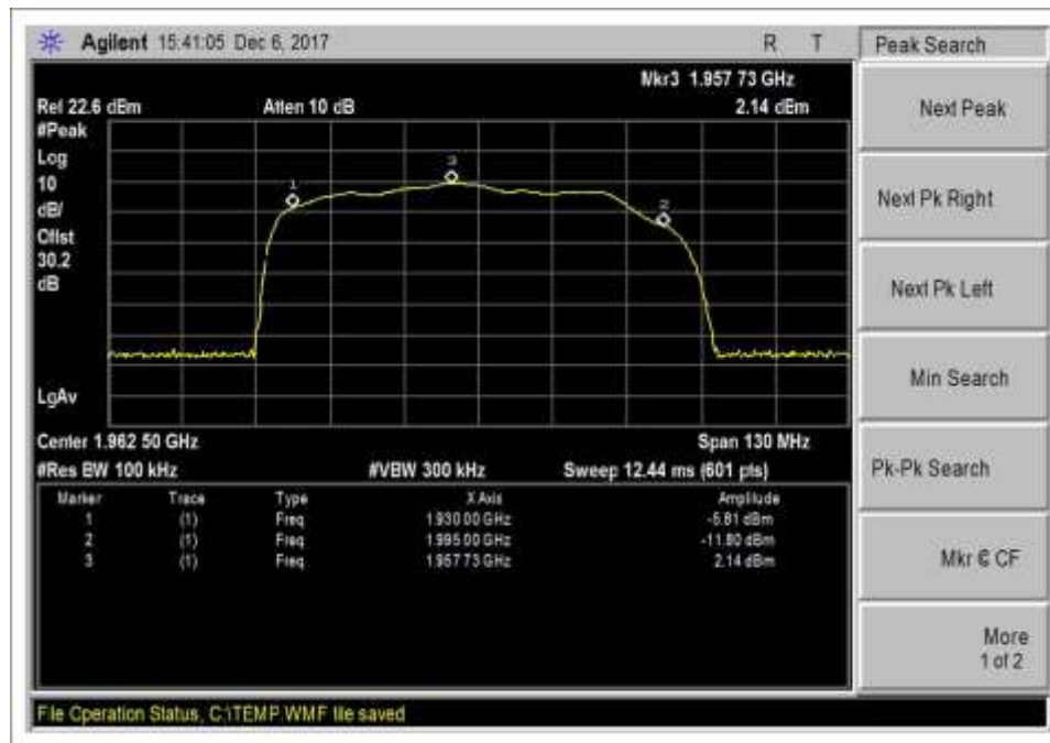
7.1 DL 1930-1995M
