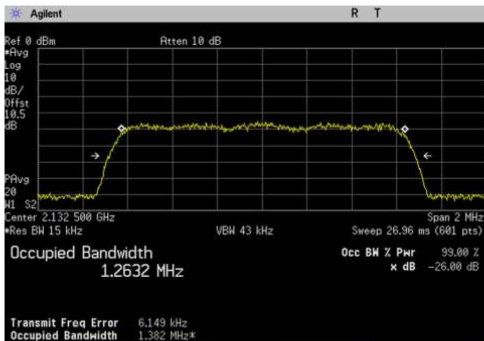
DL_2110-2155_CDMA_2132.5MHz
