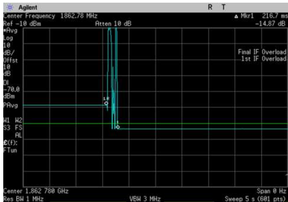
UL_1850-1915_ 1862.78MHz
