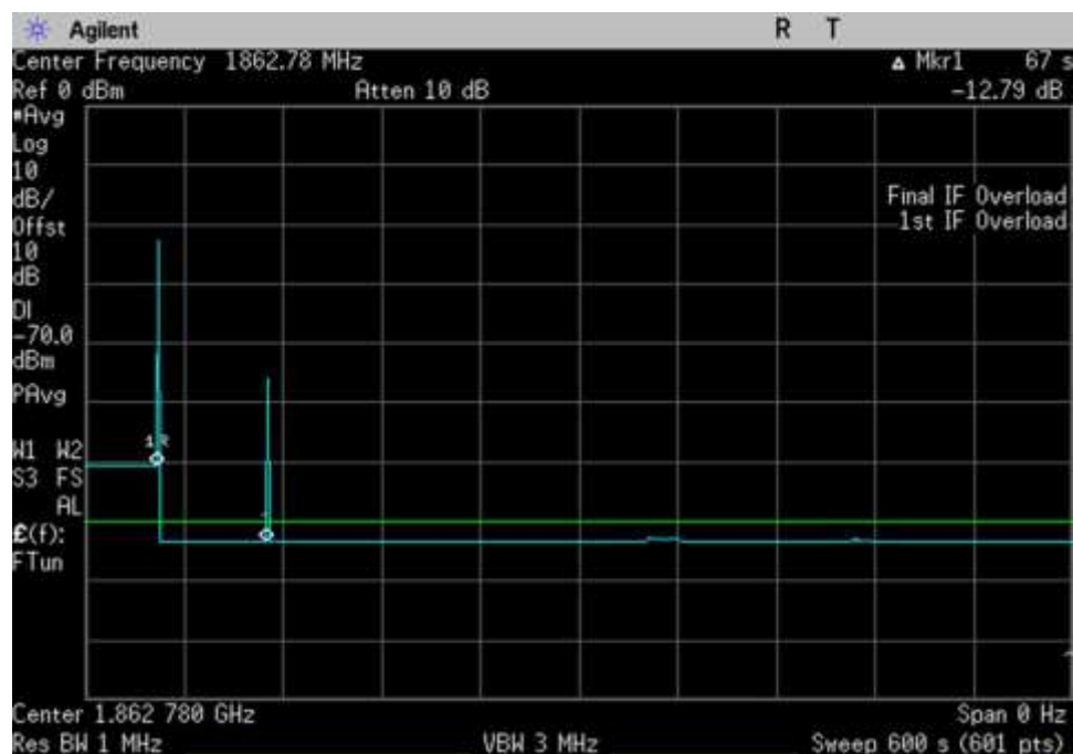
UL_1850-1915_600sec_ 1862.78MHz
