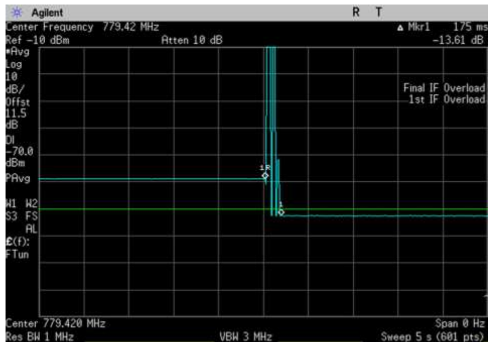
UL_776-787_779.42MHz
