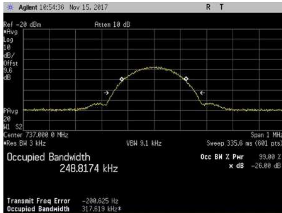
7.10_OBW_DL_728-746MHz_GSM_In
