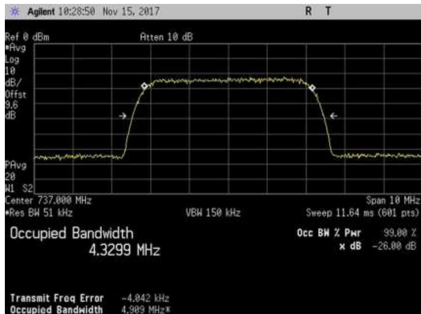
7.10_OBW_DL_728-746MHz_AWGN_Out
