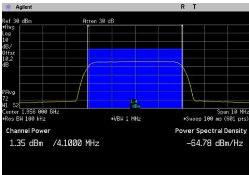
DL_1930-1995_AWGN_Max_1956MHz
