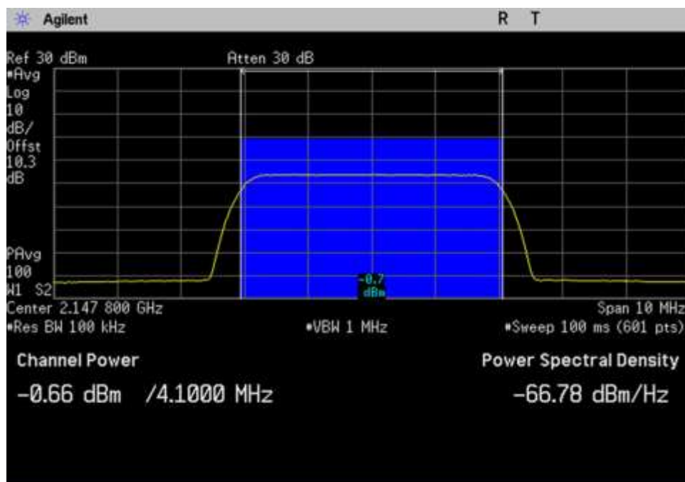
DL_2110-2155_AWGN_Max_2147.8MHz
