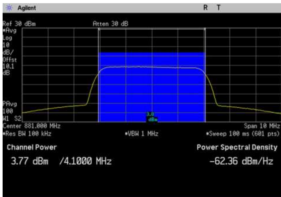
DL_869-894_AWGN_Max_ 881MHz
