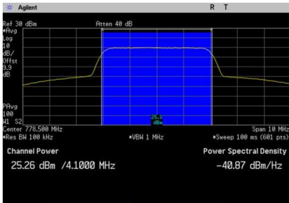
UL_776-787_AWGN_778.5MHz
