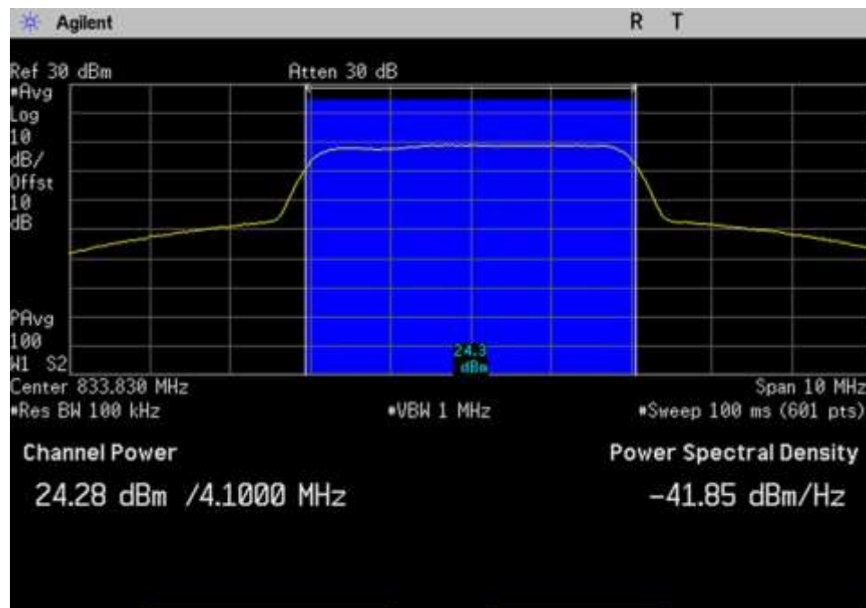
UL_824-849_AWGN_ 833.83MHz
