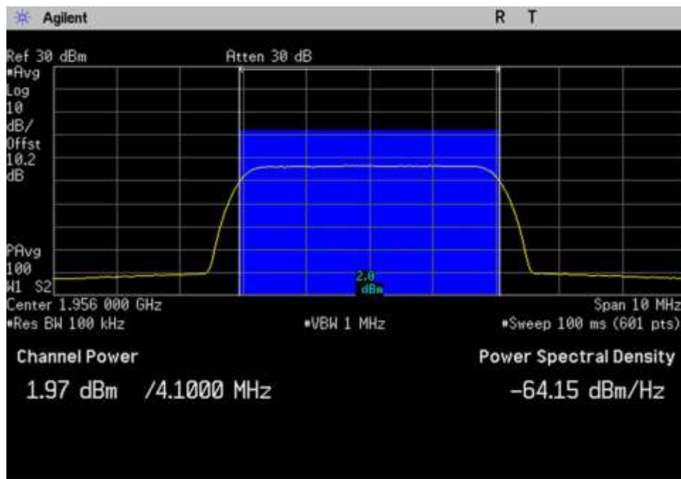
DL_1930-1995_AWGN_1956MHz
