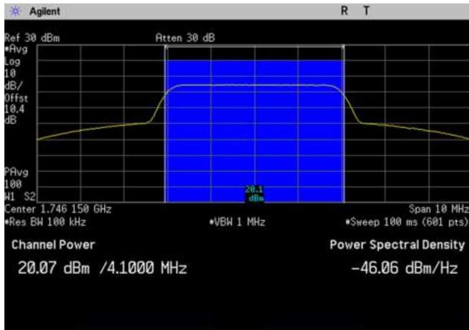
UL_1710-1755_AWGN_1746.15MHz
