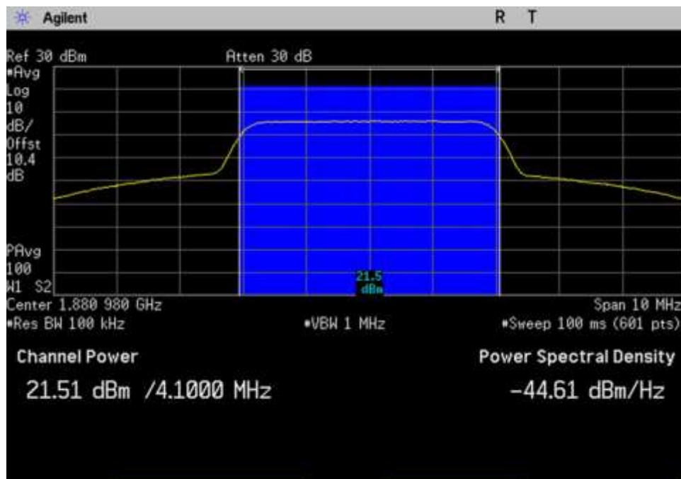
UL_1850-1915_AWGN_Max_1880.98MHz
