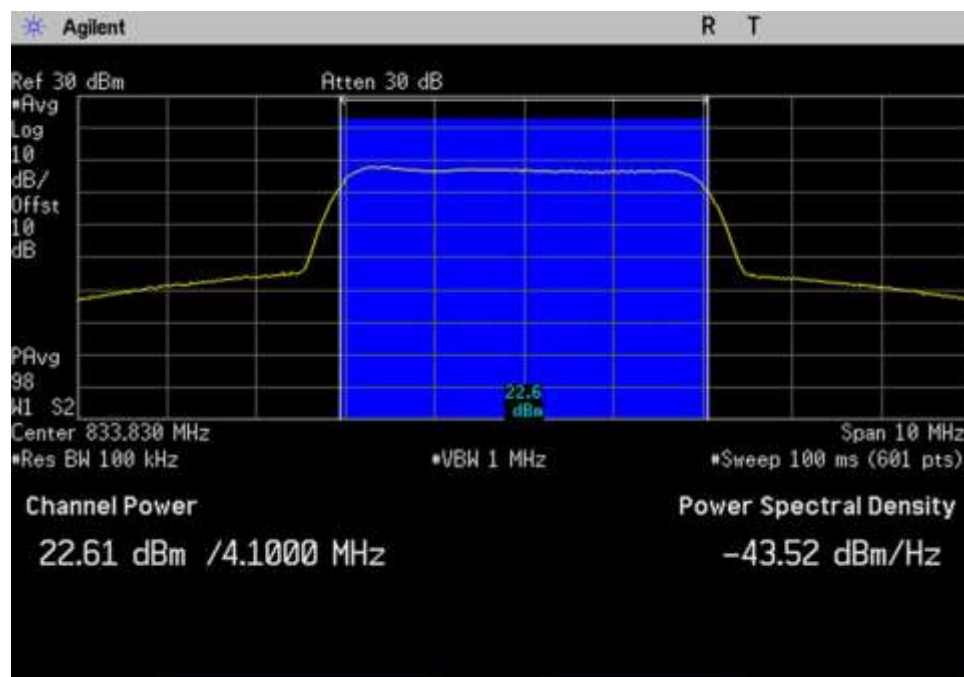
UL_824-849_AWGN_Max_ 833.83MHz
