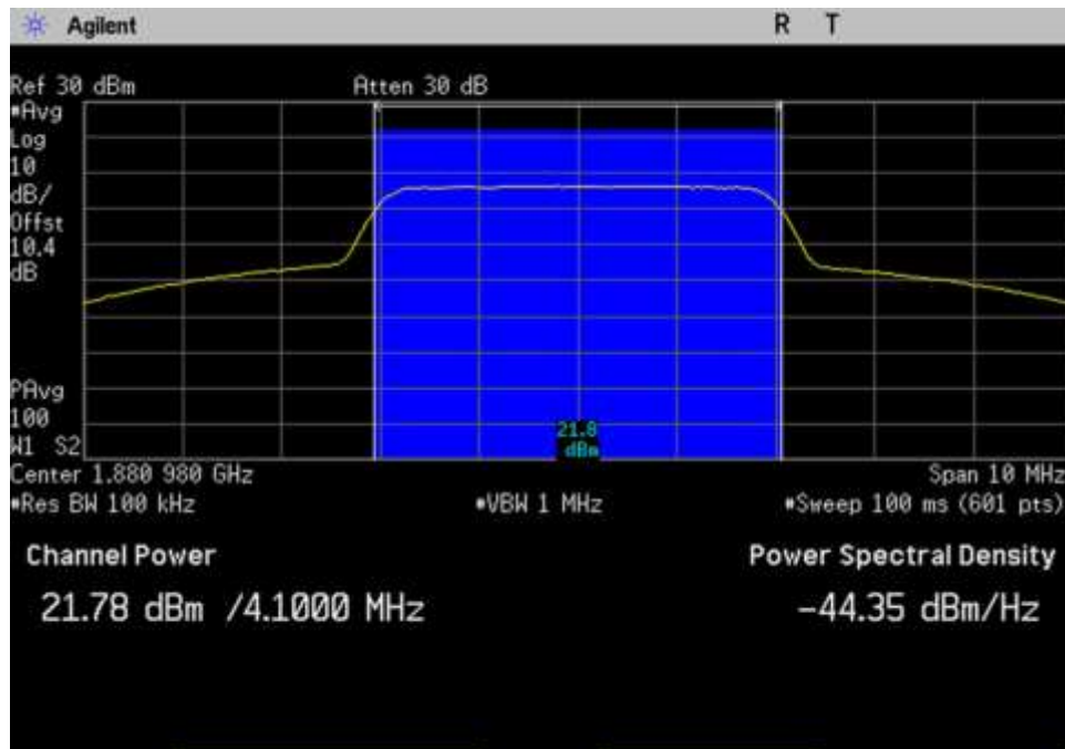
UL_1850-1915_AWGN_1880.98MHz
