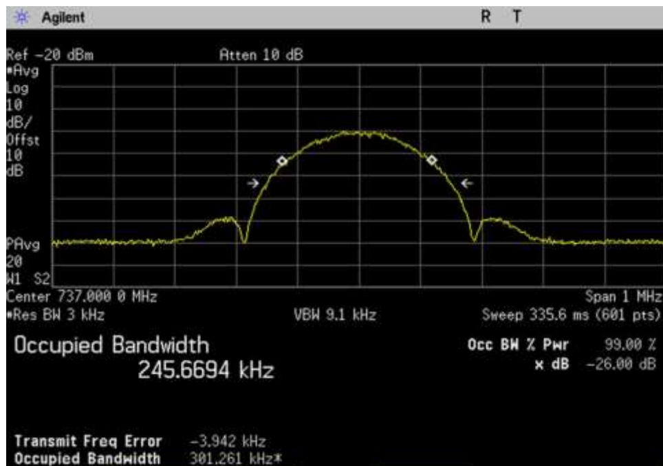
DL_728-746_EDGE_737MHz
