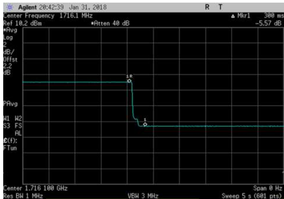
UL_1710-1755_ 1716.1MHz_timing
