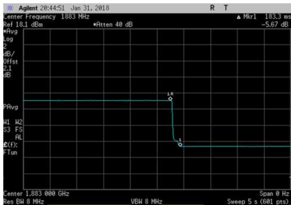
UL_1850-1915_ 1883MHz_timing
