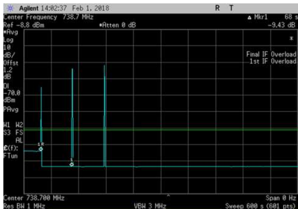
DL_728-746_600sec_ 738.7MHz
