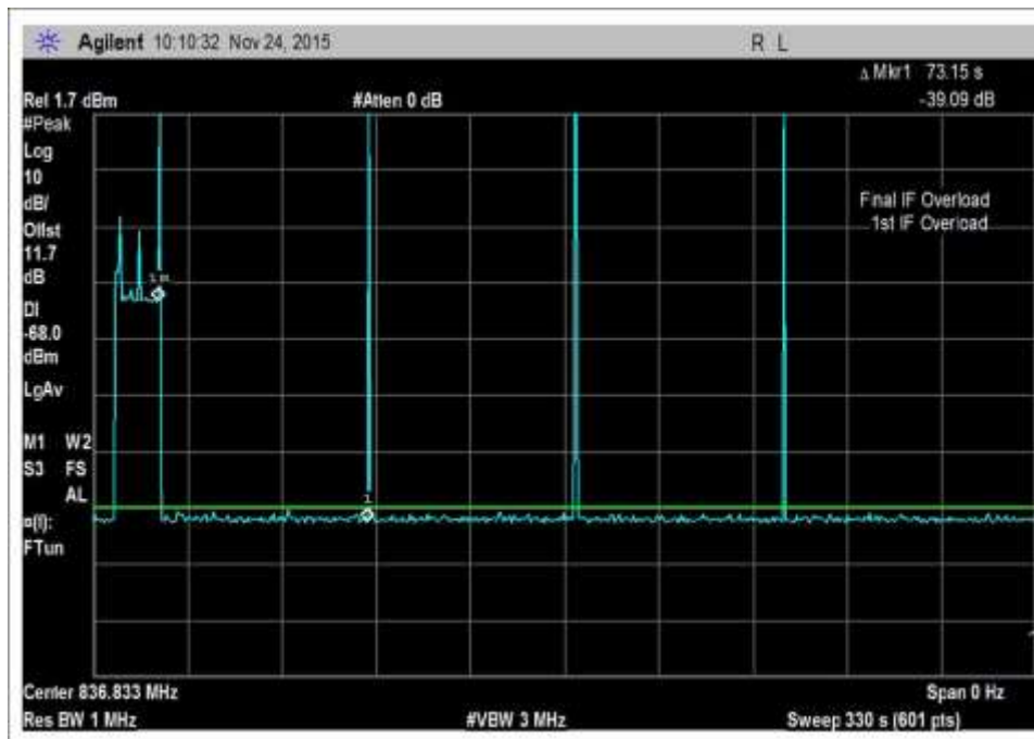
7.11_osc_UL-824-849MHz-330sec
