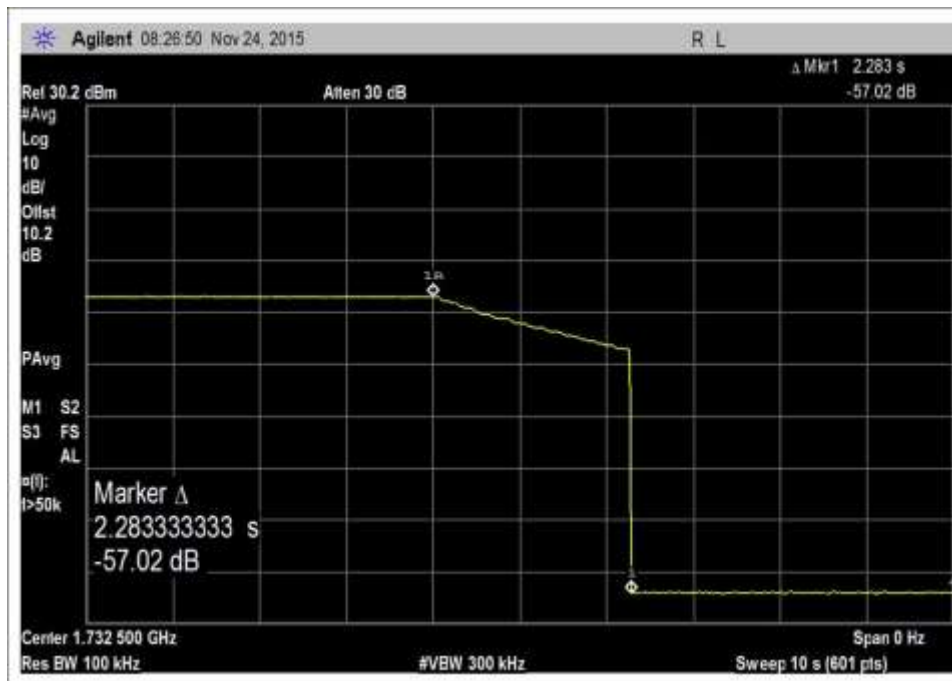
7.9.2_VarULGainTiming_UL_1710-1755MHz
