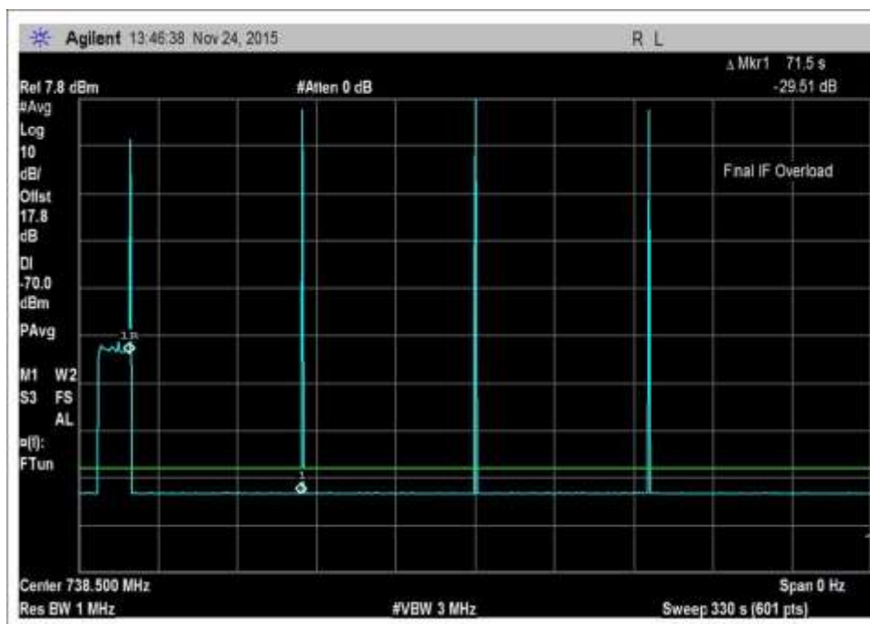
7.11_osc_DL-728-746MHz-330sec
