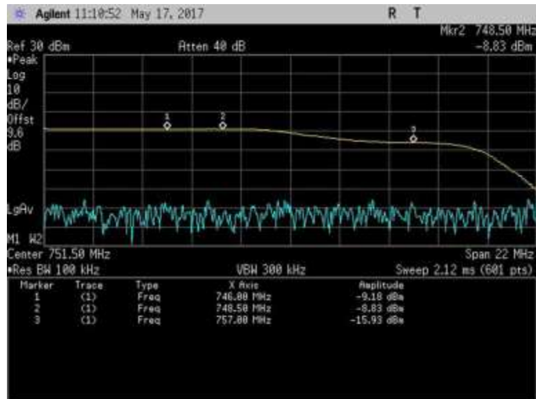
7.1_Band Verify_DL_746-757MHz
