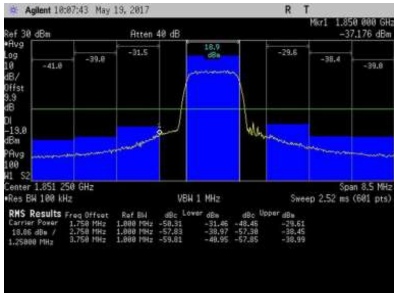
7.5_OBE_UL_1850-1915MHz_L_PreAGC_CDMA
