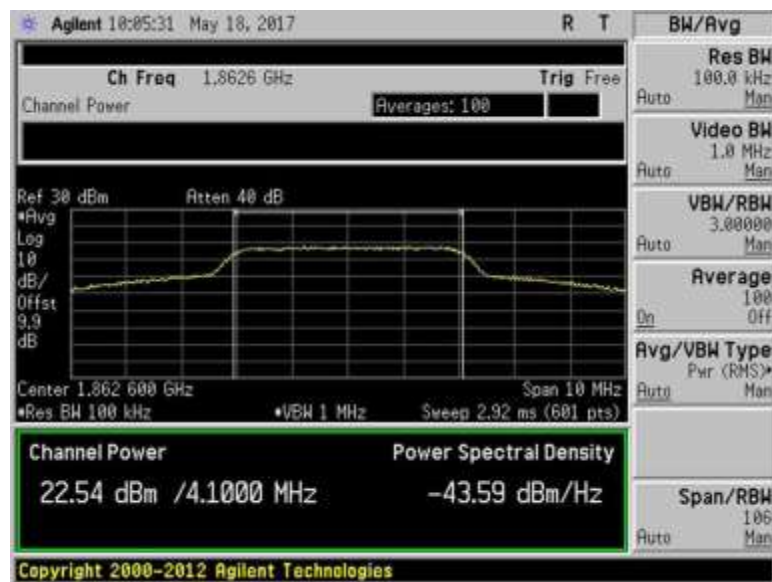
7.2_Power_UL_1850-1915MHz_AWGN_Max
