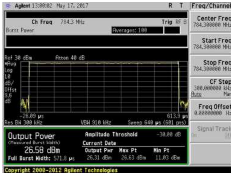
7.2_Power_UL_776-787MHz_GSM_Max
