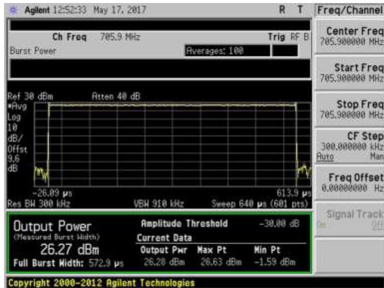
7.2_Power_UL_698-716MHz_GSM
