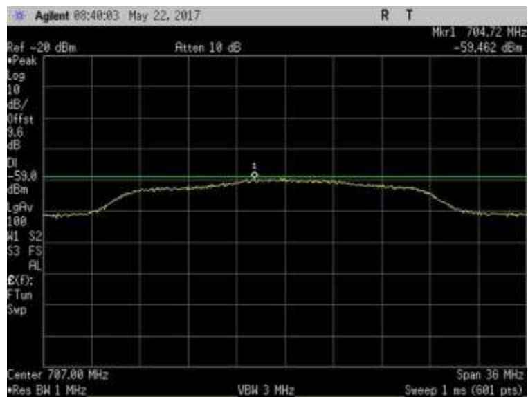
7.7.1_Noise_UL_698-716MHz
