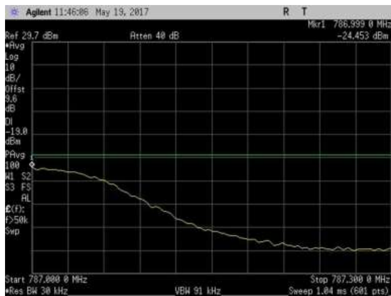
7.5_OBE_UL_776-787MHz_H_PreAGC_GSM
