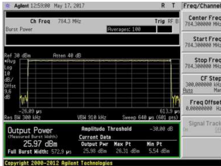
7.2_Power_UL_776-787MHz_GSM
