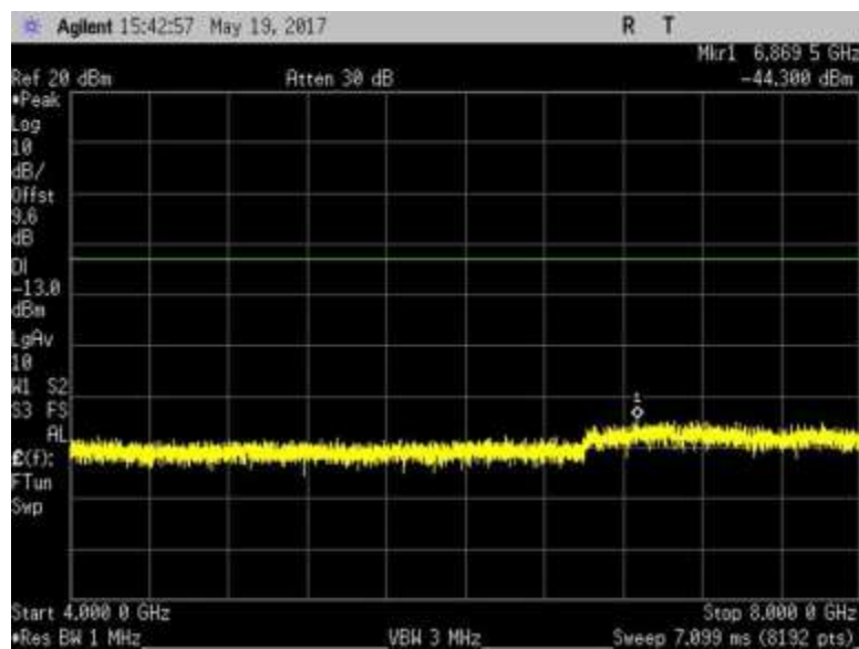
7.6_CSE_UL_776-787MHz_R2
