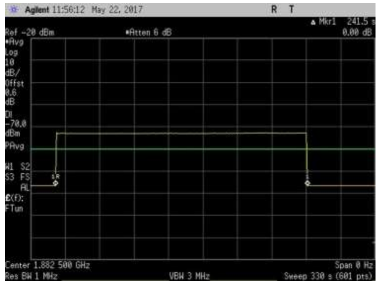
7.8_InactivityUL_1850-1915MHz
