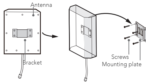
Panel-antenna installation
