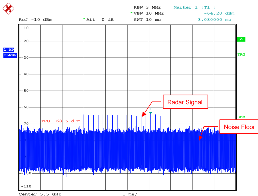
Radar Signal 3
