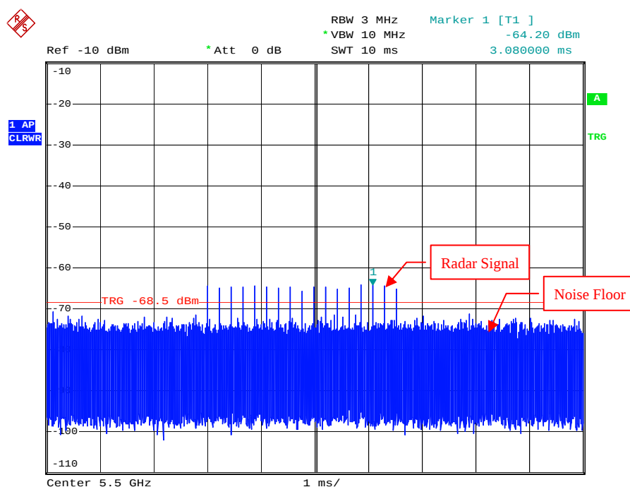
Radar Signal 3
