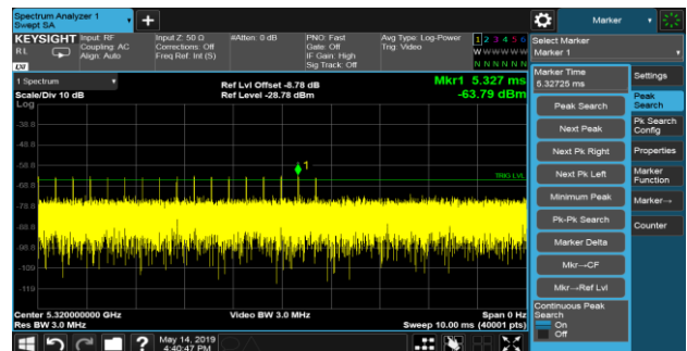
Radar Type 5 Calibration Plot
