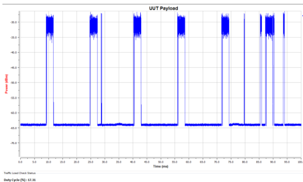
5310MHz, 802.11ac VHT40, Band 2 Time On/ (Time On + Off Time) =17.31%
