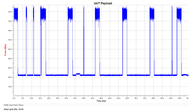
5500MHz, 802.11ac VHT20, Band 3 Time On/ (Time On + Off Time) =19.45%
