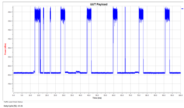
5510MHz, 802.11ac VHT40, Band 3 Time On/ (Time On + Off Time) =17.31%
