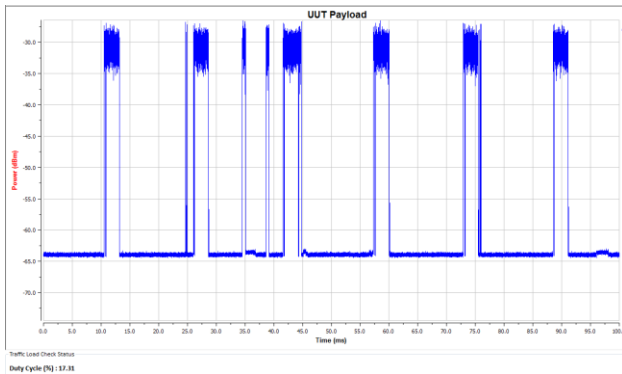
5320MHz, 802.11ac VHT20, Band 2 Time On/ (Time On + Off Time) =17.31%
