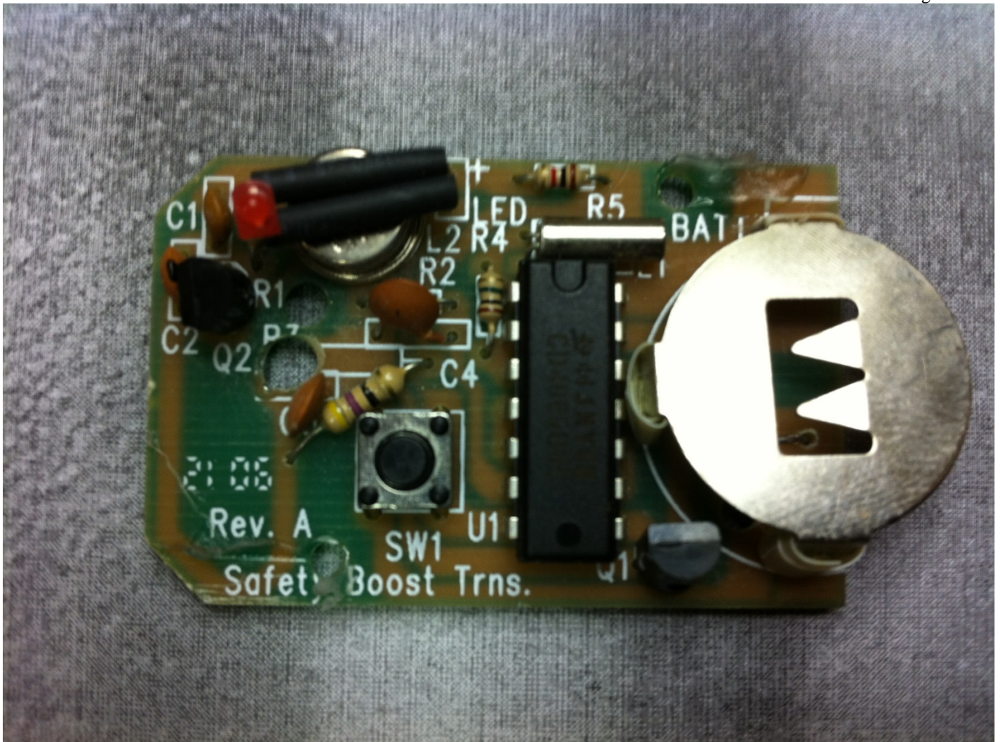
Figure 1 Circuit Card Assembly - Top View (Component Side)
