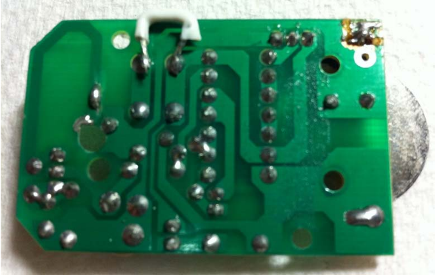
Figure 2 Circuit Card Assembly - Bottom View (Etch Side)
