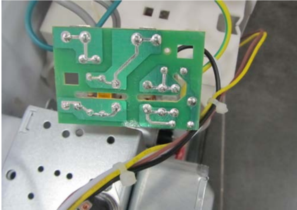
Power Filter Board Bottom View
