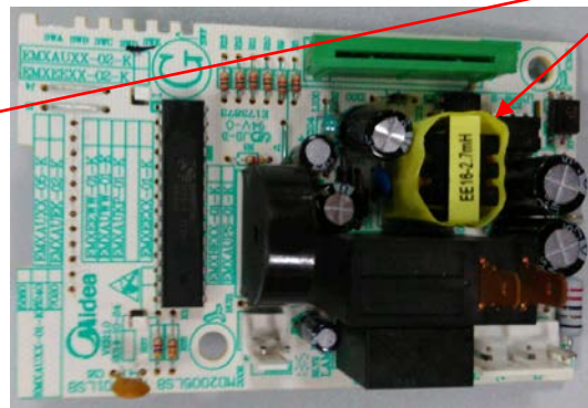
New Mother board –top view
