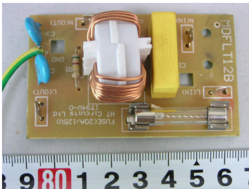
EUT – Filter PCB Top View
