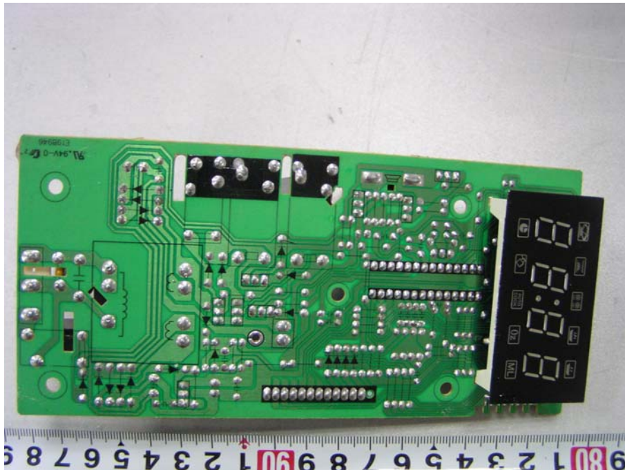
EUT – Display and Button PCB Bottom View
