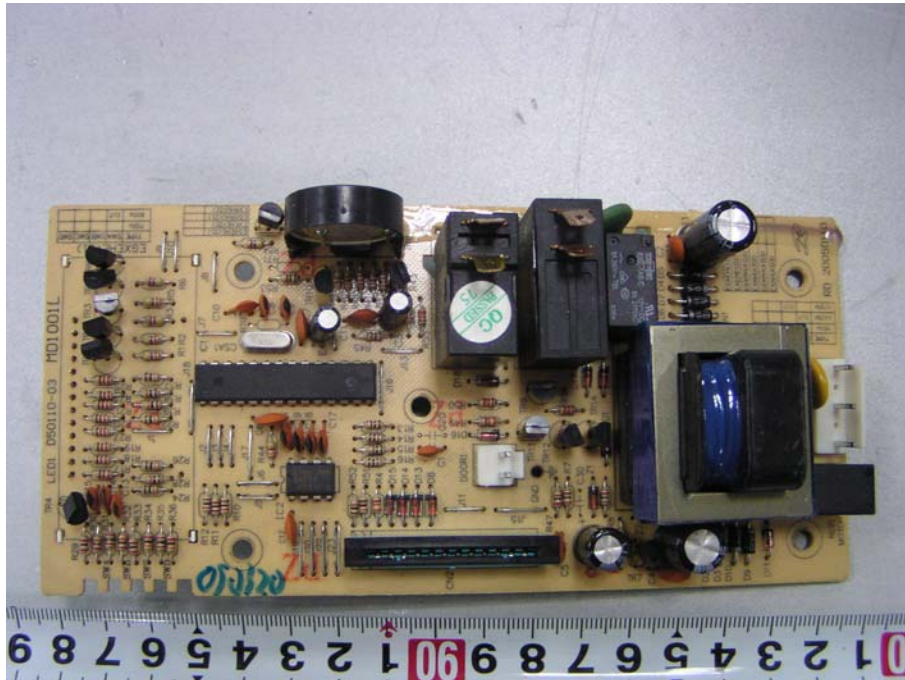
EUT – Display and Button PCB Top View
