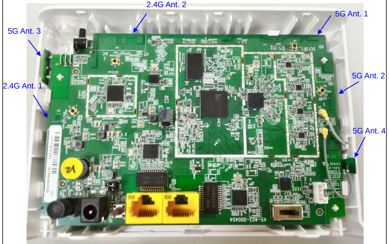
Antenna location
