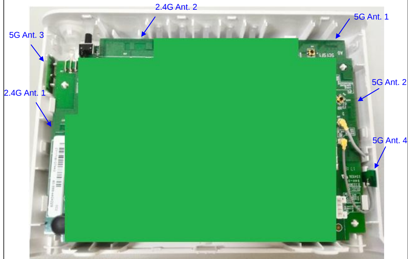
Antenna location
