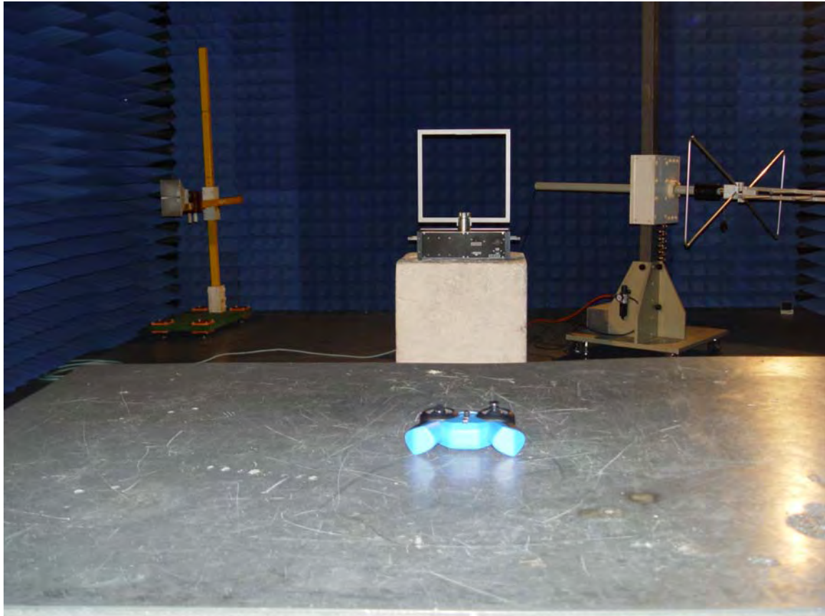
Radiated emissions test 9 KHz - 30 MHz
