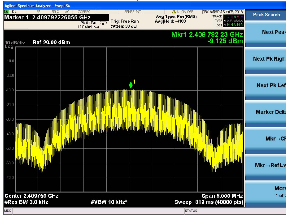
DSSS PSD plot on channel 1
