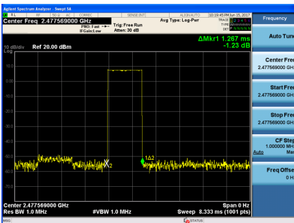
Package Transfer Time Plot CH36
