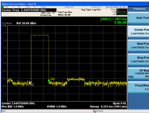
Package Transfer Time Plot CH18
