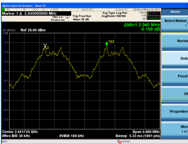
Channel Separation plot on channel 17-18
