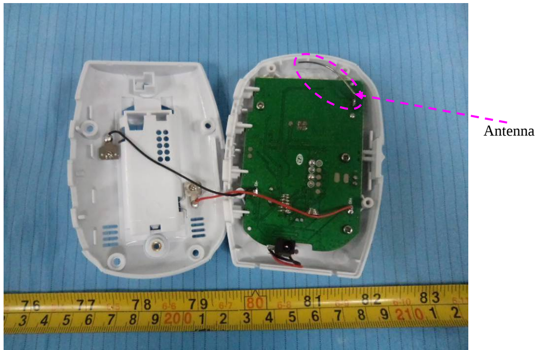
EUT (Parent Unit) – Cover off View
