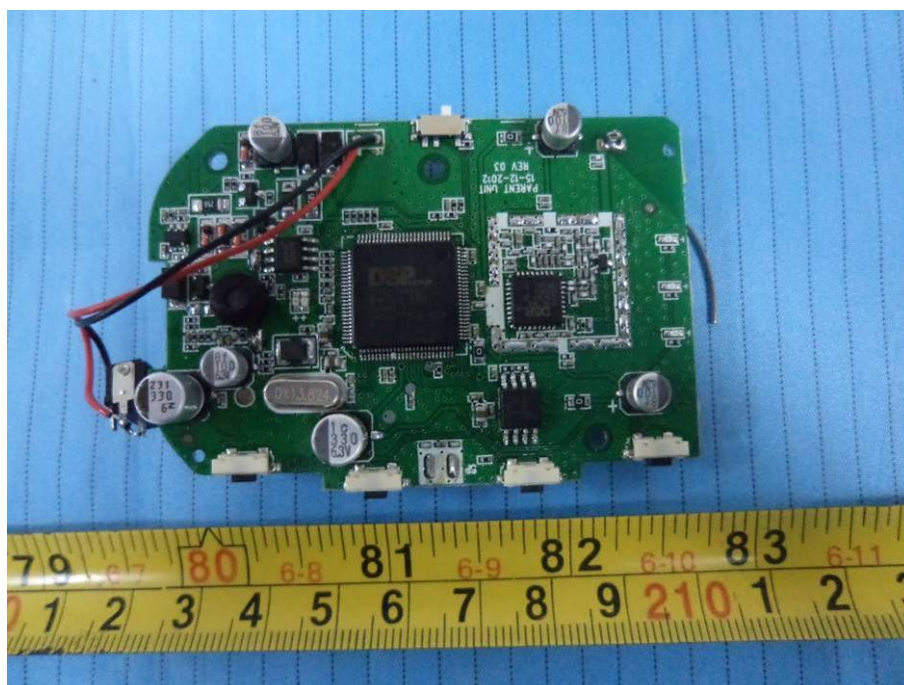
EUT (Parent Unit) – Main Board Top Shielding off View
