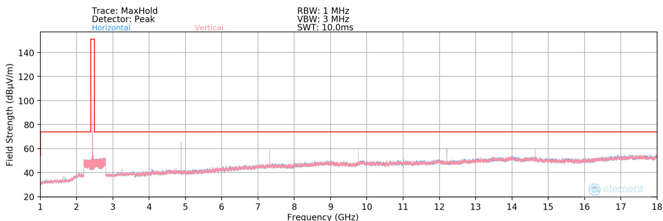
Plot 7-34. Radiated Spurious Plot above 1GHz (BT- Ch. 39)
