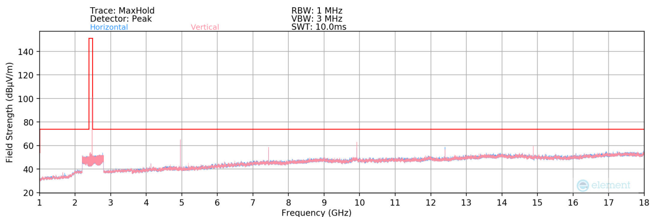
Plot 7-35. Radiated Spurious Plot above 1GHz (BT- Ch. 78)
