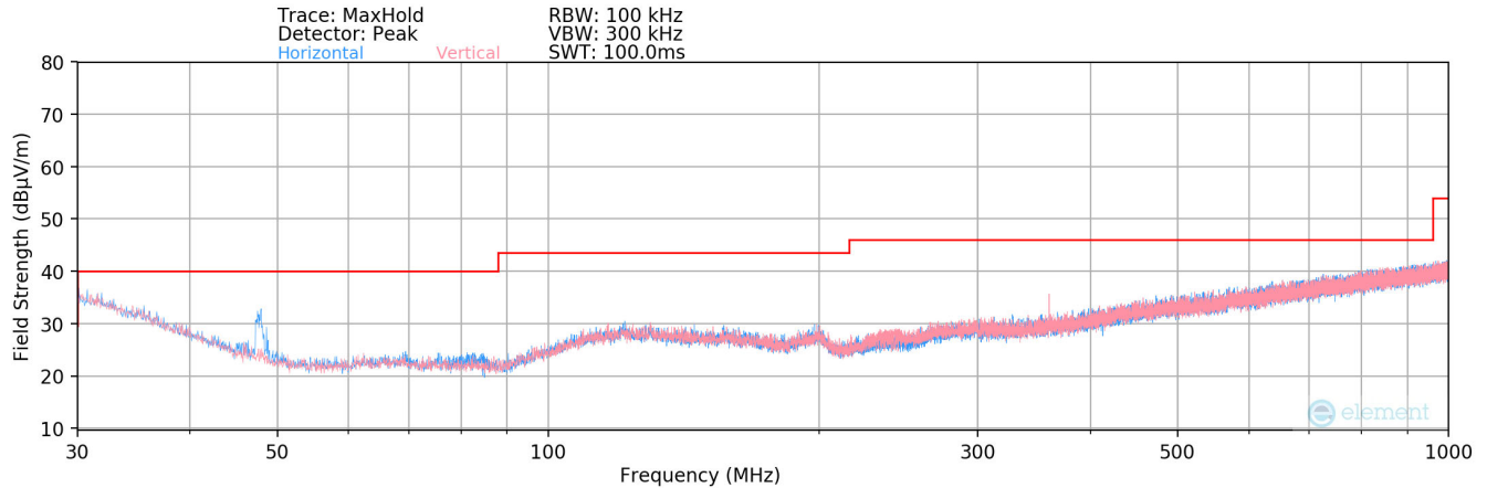
Plot 7-39. Radiated Spurious Plot below 1GHz
