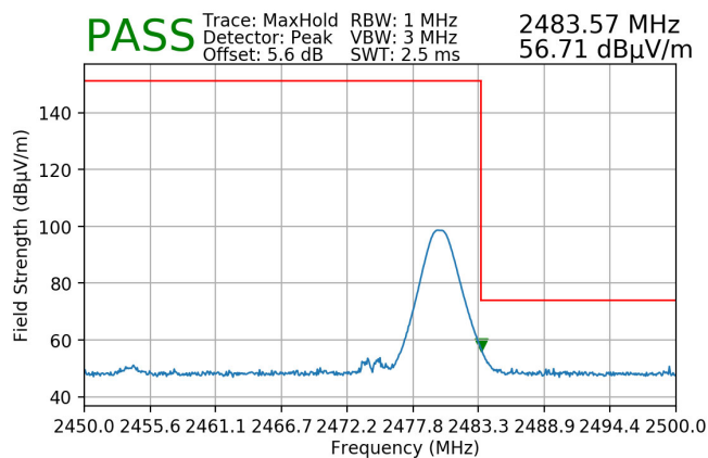
Plot 7-38. Radiated Restricted Upper Band Edge Measurement (Peak)
