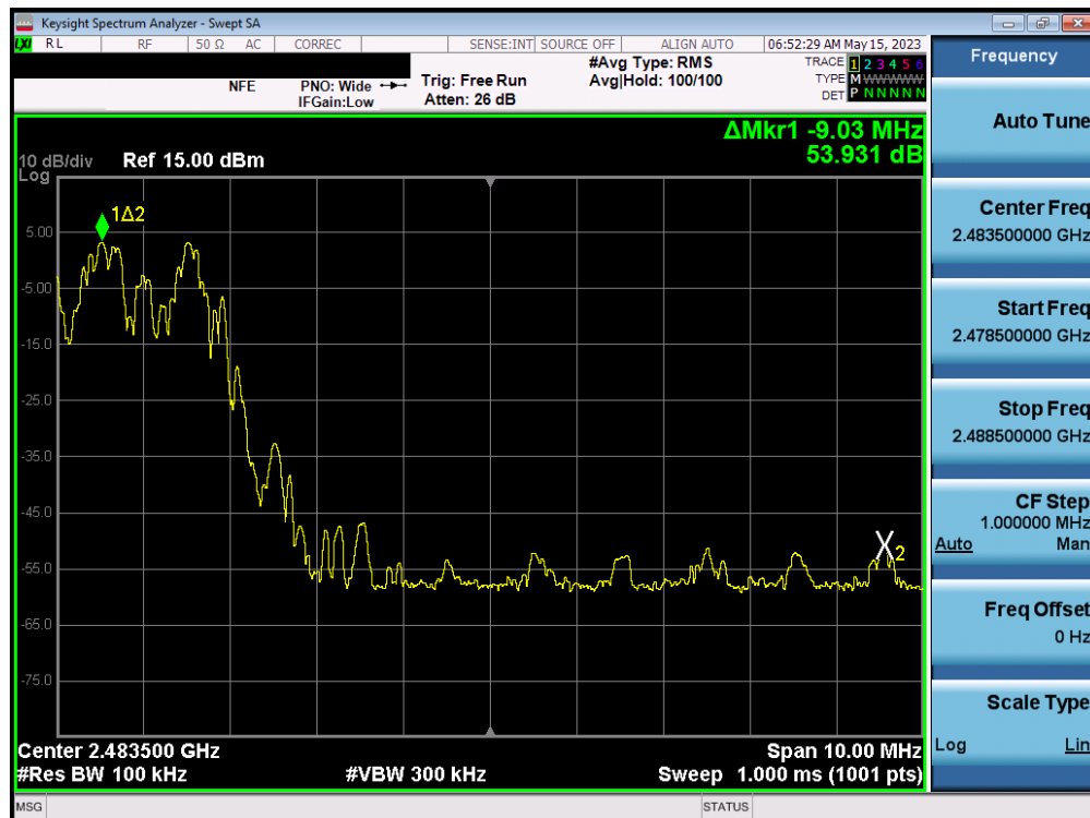
Plot 7-22. Band Edge Plot (Bluetooth with Hopping Enabled, 3 Mbps)
