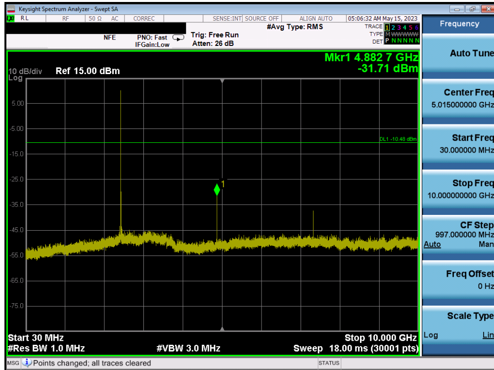
Plot 7-29. Conducted Spurious Plot (Bluetooth, 1Mbps – Ch. 39)
