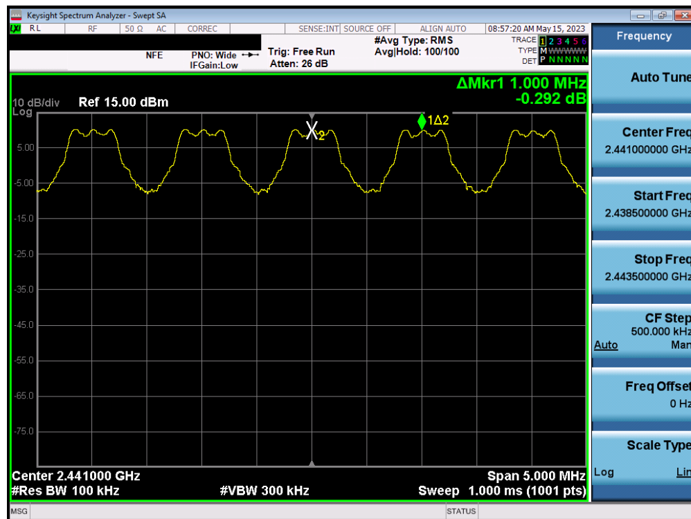
Plot 7-23. Channel Spacing Plot (Bluetooth)
