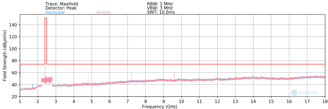
Plot 7-33. Radiated Spurious Plot above 1GHz (BT- Ch. 0)
