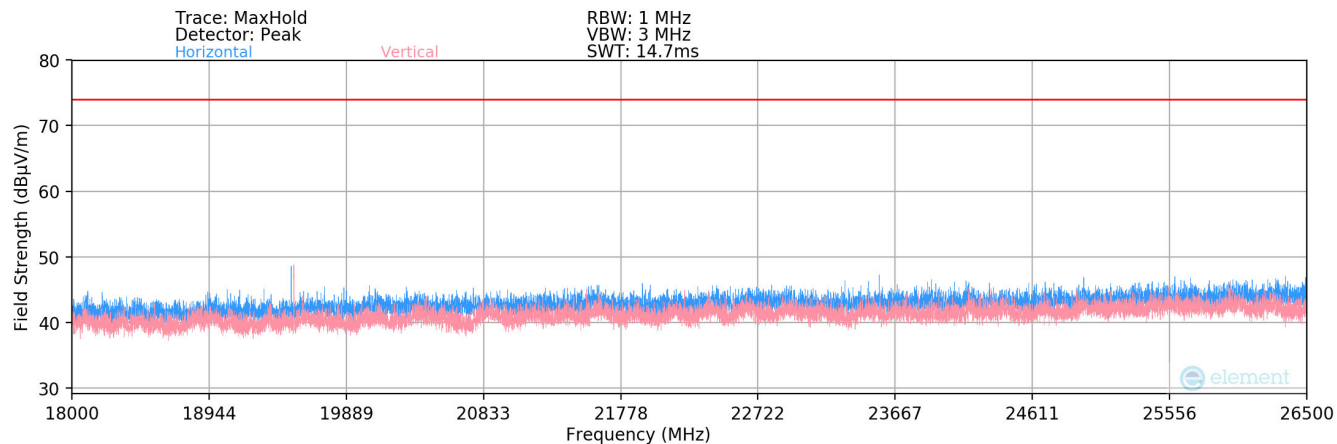
Plot 7-36. Radiated Spurious Plot above 18GHz
