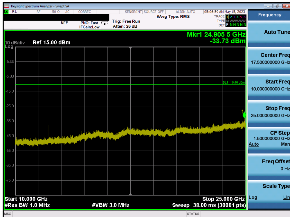
Plot 7-30. Conducted Spurious Plot (Bluetooth, 1Mbps – Ch. 39)
