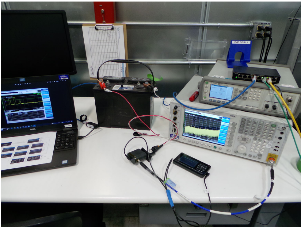
Configuration 5: Roady BT Radio Bluetooth Mode Conducted Emissions
