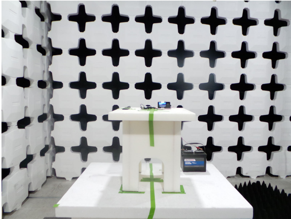
Configuration 5: Rody BT Radio Bluetooth Mode Radiated Emissions below 18GHz front
