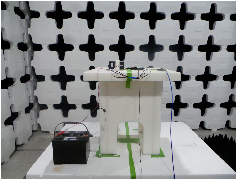
Configuration 5: Rody BT Radio Bluetooth Mode Radiated Emissions below 18GHz rear
