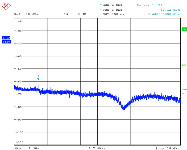
Plot 6-29. Radiated Spurious Plot above 1GHz (Ant. Pol. H, High Channel – 107.9MHz)
