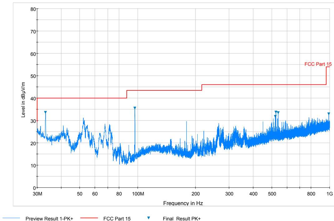
Plot 6-16. Radiated Spurious Plot below 1GHz (Pol. V, Mid Channel – 96.9MHz)
