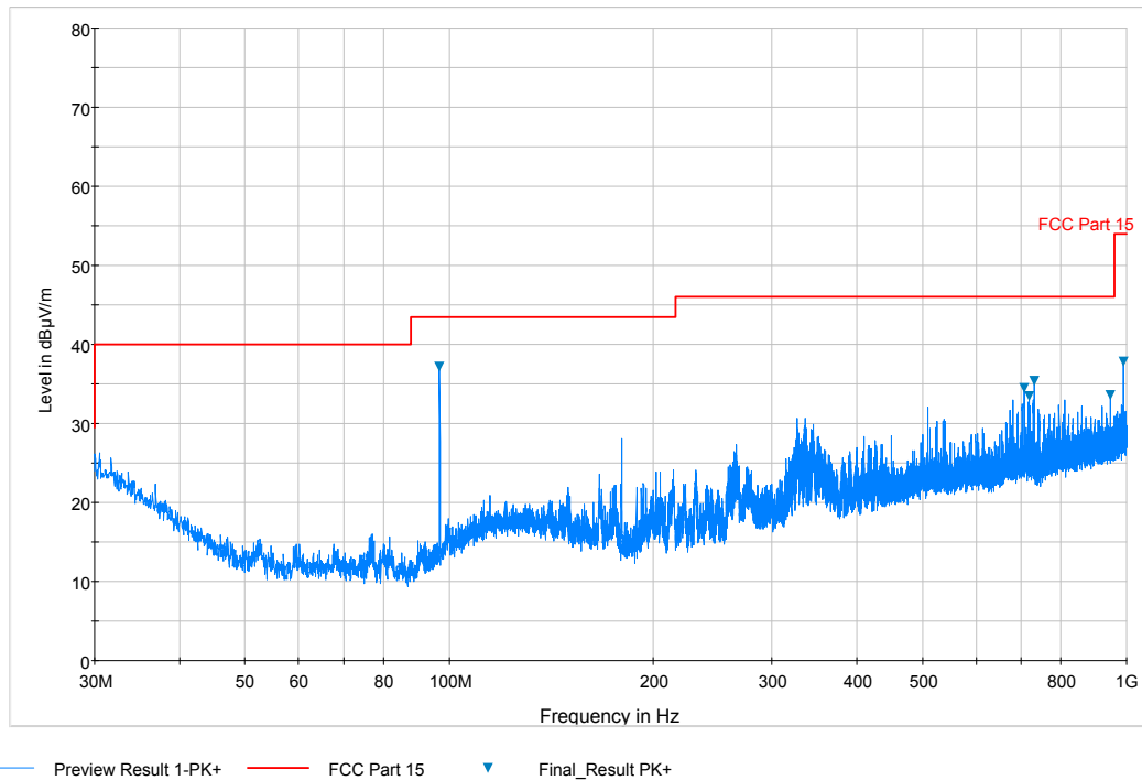
Plot 6-15. Radiated Spurious Plot below 1GHz (Pol. H, Mid Channel – 96.9MHz)
