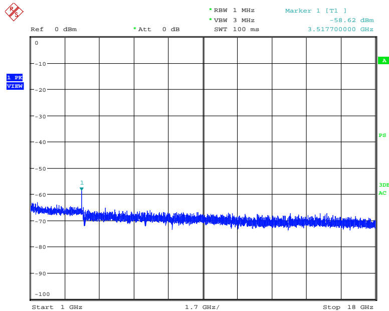
Plot 6-31. Radiated Spurious Plot above 1GHz (Ant. Pol. H, Low Channel – 88.1MHz)
