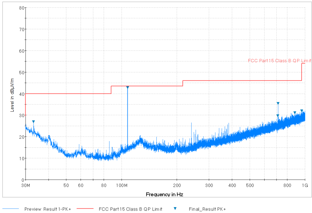
Plot 6-23. Radiated Spurious Plot below 1GHz (Pol. H, High Channel – 107.9MHz)
