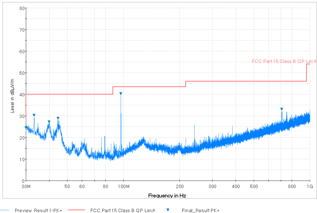
Plot 6-22. Radiated Spurious Plot below 1GHz (Pol. V, Mid Channel – 96.9MHz)
