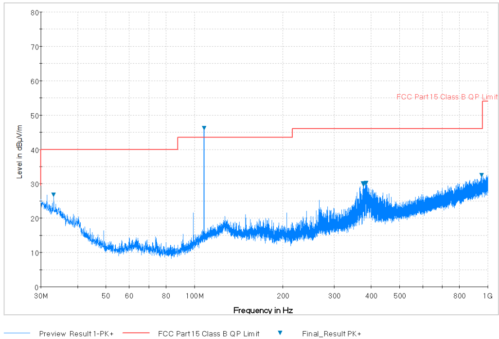
Plot 6-17. Radiated Spurious Plot below 1GHz (Pol. H, High Channel – 107.9MHz)
