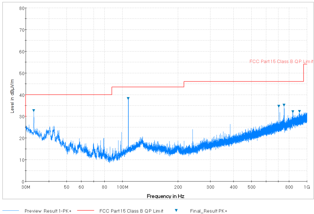
Plot 6-24. Radiated Spurious Plot below 1GHz (Pol. V, High Channel – 107.9MHz)
