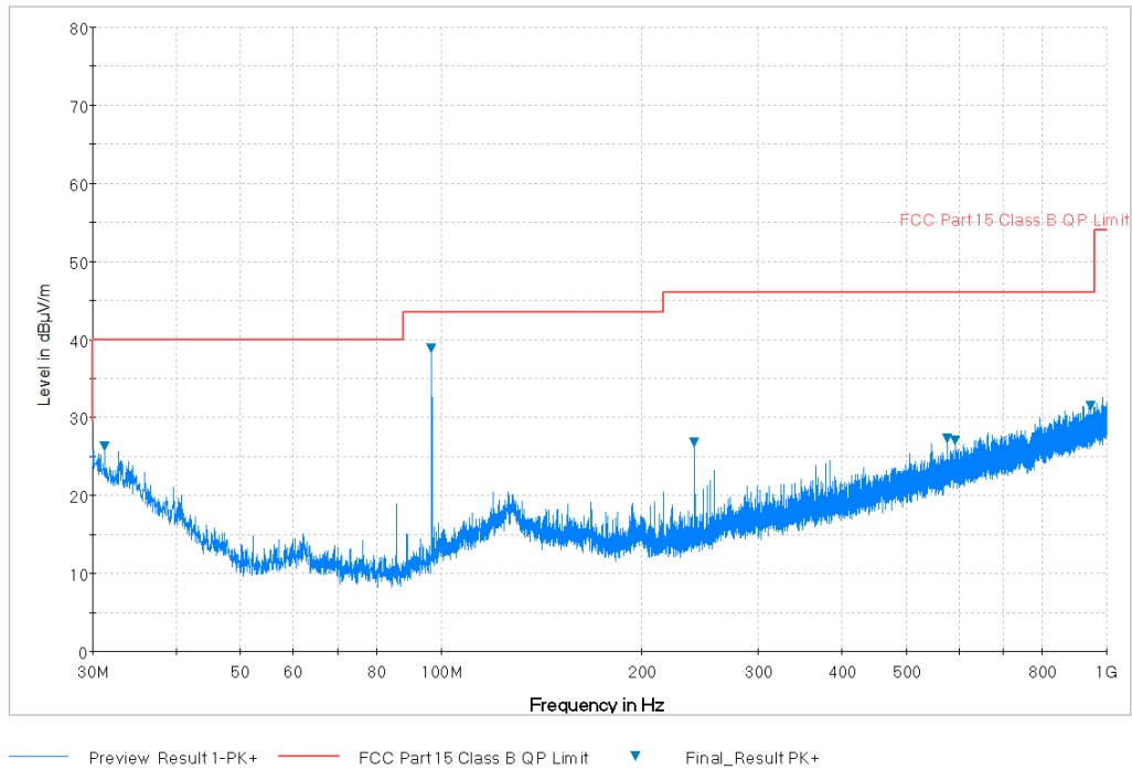
Plot 6-21. Radiated Spurious Plot below 1GHz (Pol. H, Mid Channel – 96.9MHz)
