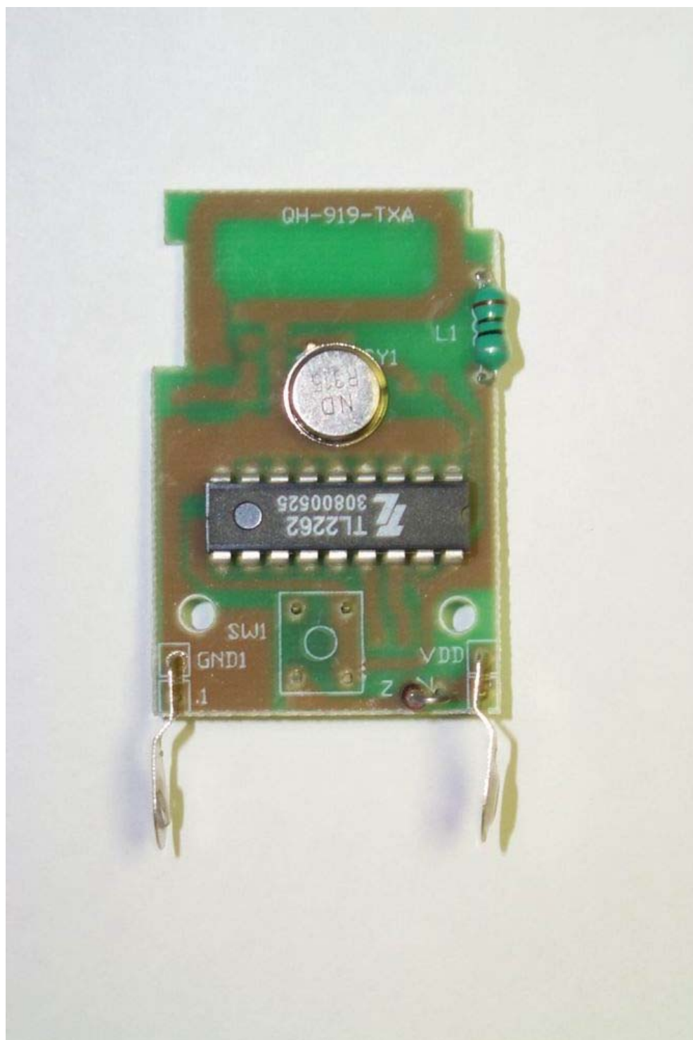
Component Side
