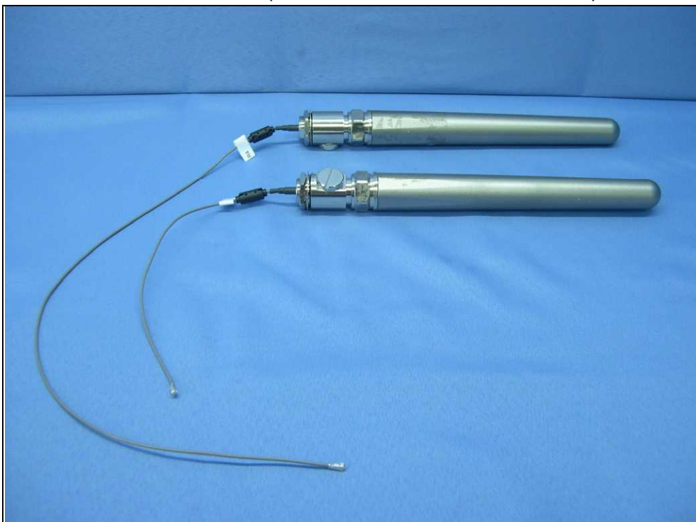
EUT + Antenna (without filter, Gain: 4.6dBi / 4dBi)
