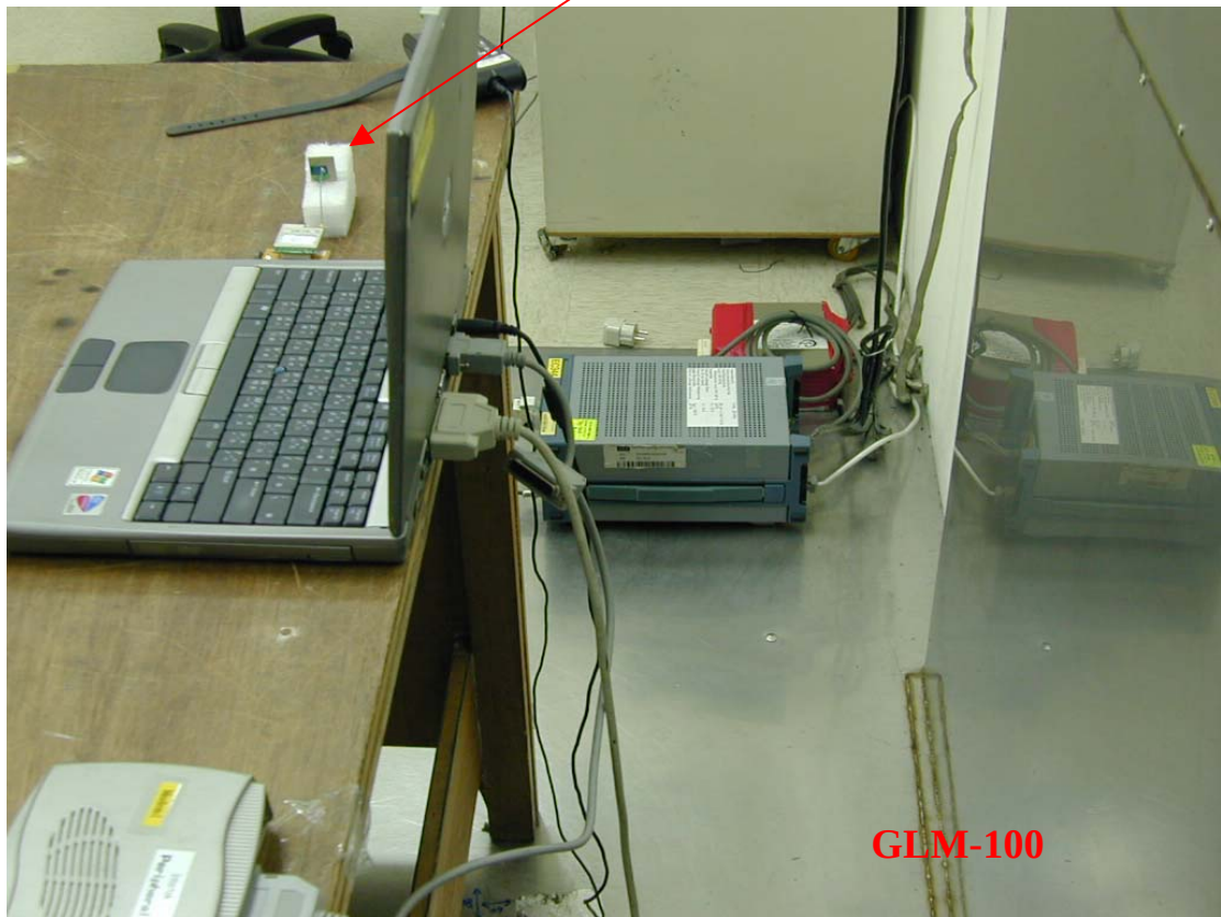
Photo 5: Conducted Emission Test set-up photo (PCB Antenna)
