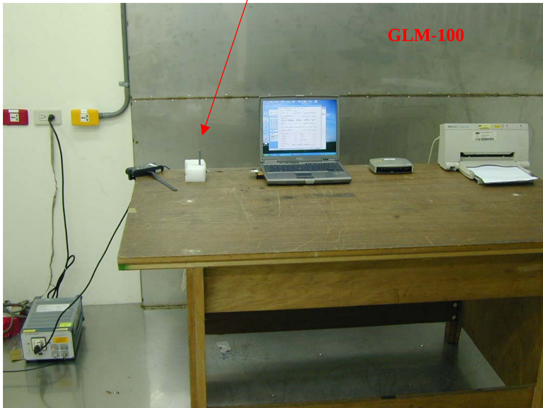
Photo 1: Conducted Emission Test set-up photo (Dipole Antenna)
