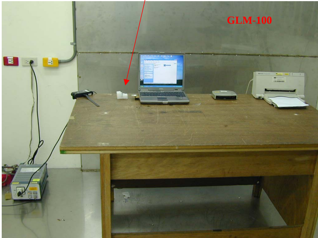
Photo 4: Conducted Emission Test set-up photo (PCB Antenna)
