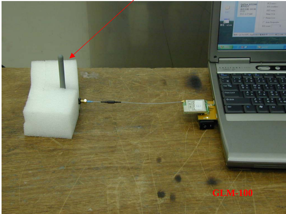
Photo 3: Conducted Emission Test set-up photo (Dipole Antenna)
