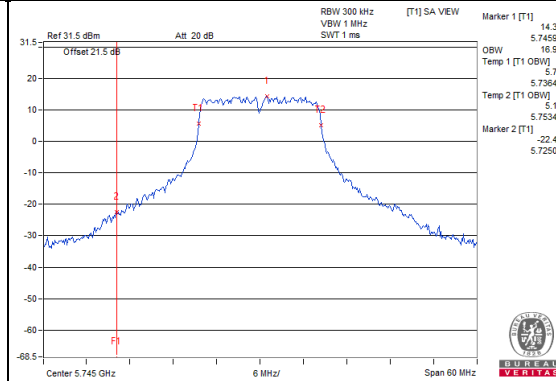
802.11a_Chain 3 / CH149
