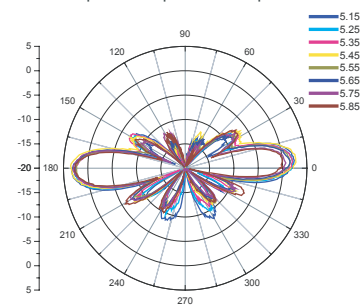
E-plane Co-polarization pattern
