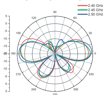
E-plane Co-polarization pattern
