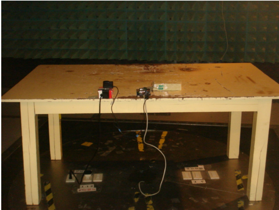
EUT work with Antenna C&D
